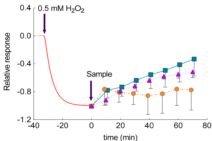
Figure 7. Relative, average amperometric current response of skin covered oxygen electrode immersed in CBS, pH 5.5, to addition of H_2O_2 (0.5 mM, red dotted and solid lines, n = 13 ) CA sol (CA 0.5 mM, triangle, n = 3 ); CA-ETHO (CA 0.5 mM, square, n = 6 ) and unloaded ETHO (circles, n = 4 ).
