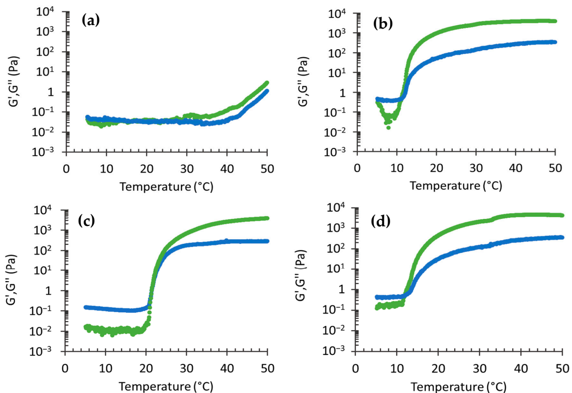
Figure 5. Effect of the temperature on storage ( G' , green) and loss ( G'' , blue) moduli for ETHO (a), ETHO-pol (b), CA-pol (c), and CA-ETHO-pol (d).
