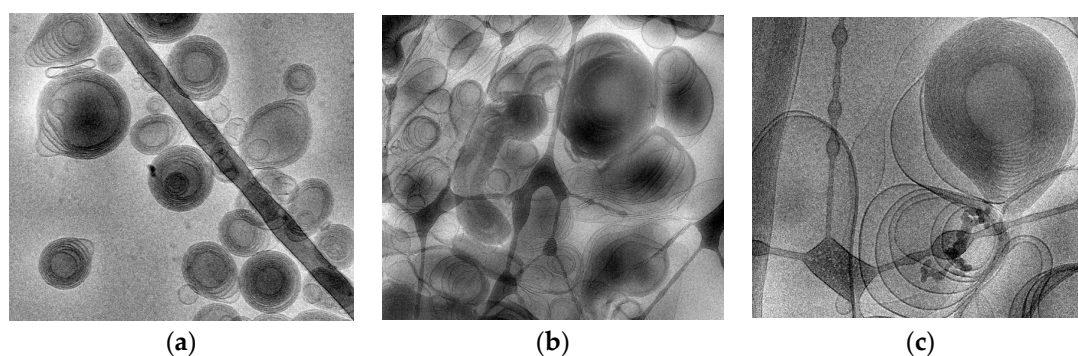
Figure 2. Cryo-transmission electron microscopy images (Cryo-TEM) of CA-ETHO (a) and CA-ETHO-pol (b,c). Bar corresponds to 200 nm (a,b) or 100 nm (c).
