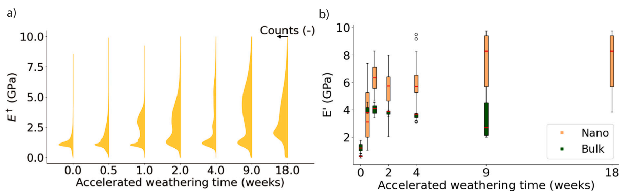
Fig. 6. (a) Effective young's modulus histogram evolution over accelerated weathering duration measured with ImAFM. For ImAFM every measured pixel corresponds to a calculated effective Young's-modulus. The number of counts (pixels) per effective Young's modulus are normalized for each sample and presented in the violin plot for each time point. With increasing weathering time the Young's modulus not only increases but also is spread more widely. (b) Storage modulus evolution over accelerated weathering time at 20 °C and approx. 150 Hz. Two different measurement methods are presented: Bulk DMA measurements as described in Section 2.4 and VEA as described in Section 2.3. With increasing accelerated weathering time the storage modulus increases.
