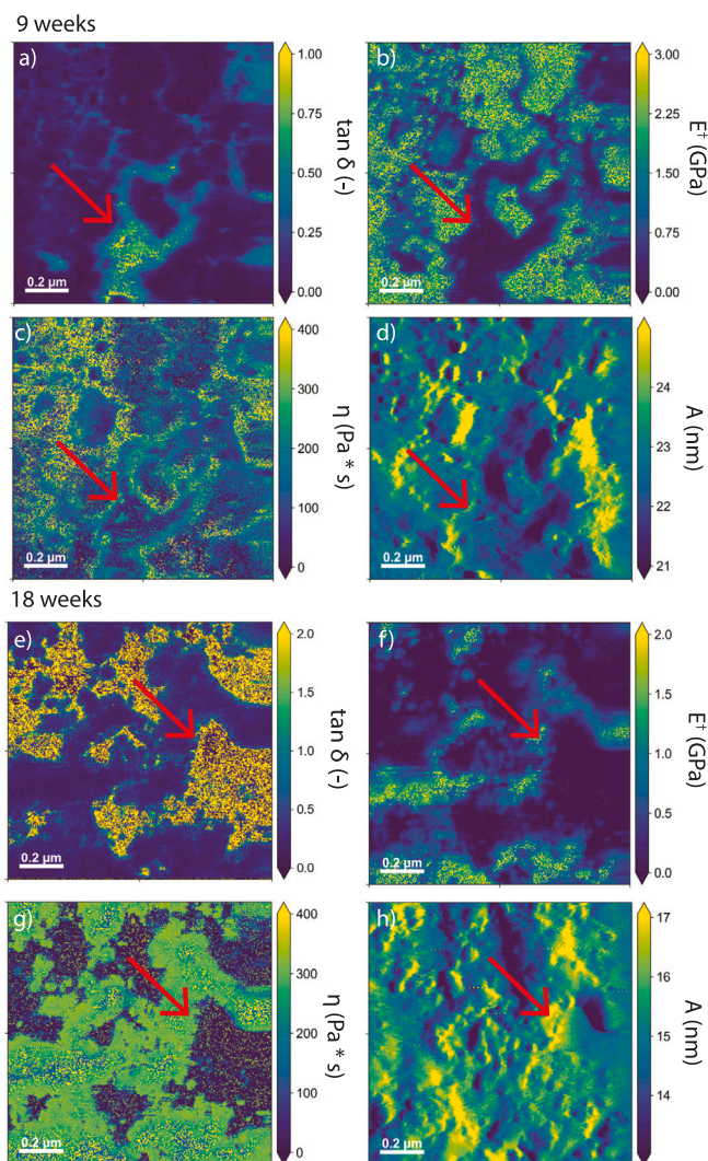
Fig. 5. 1\ \mu\text{m} \times 1\ \mu\text{m} images of highly damped areas which were first detected after 9 weeks (a–d) and are more pronounced after 18 weeks (e–h) of accelerated weathering. The arrow marks the same areas in the loss tangent \tan \delta (a+e), E-modulus (b+f), viscosity (c+g) and cantilever amplitude (d+h) of the first drive tone of ImAFM measurement for 9 and 18 weeks weathering duration.
