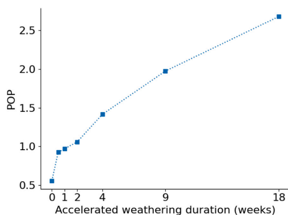
Fig. 7. FTIR measurements of the accelerated weather samples. With increasing weathering time the amount of photo-oxidation products (POP) increases which leads to more polar groups in the coating molecular structure. The inclusion of dashed lines in the diagrams is intended to facilitate the visual guidance of the reader's eye. For more details see Section 2.6.
