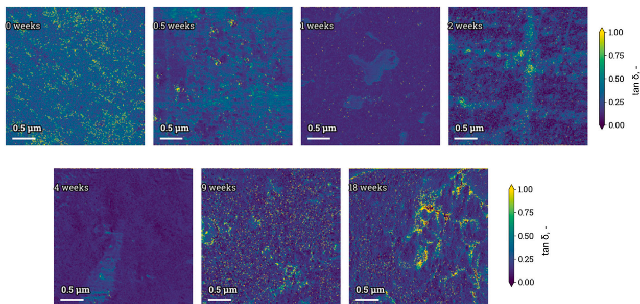
Fig. 4. Spatial distribution of the loss tangent \tan \delta evolution over accelerated weathering duration. With increasing weathering time areas with high damping properties (high loss tangent values, yellow) appear.
