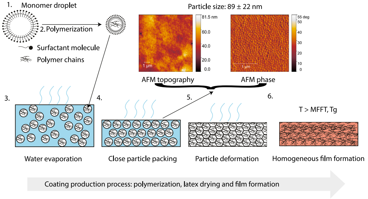
Fig. 1. Waterborne acrylate latex coating curing process. First monomer droplets are dispersed into water using a surfactant. Inside the droplets, which have a size of approximately 100–200 nm, the polymerization (step 2) takes place. Step 3–6 show the film formation process. By heating the film over T_g , polymer chain connection between the former particles are created. The AFM pictures show the topography and AFM cantilever phase of the binder before step 5 and 6.
