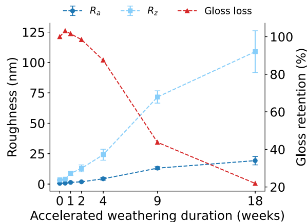
Fig. 3. Roughness values R_a and R_z and gloss loss (initial value amounts to 64 GU) over accelerated weathering duration (estimated via AFM — see Section 2.3 and quantified using a specular glossmeter — see Section 2.5). With increasing weathering duration the surface roughness increases and the gloss decreases.
