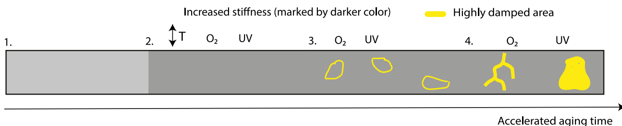
Fig. 8. Schematic representation of the proposed degradation evolution during accelerated weathering of a waterborne acrylate latex coating (top view; not to scale). The first step represents the initially homogeneous state after the curing process described in Fig. 1. During the accelerated weathering cycle, heating (step 2) induces physical aging and a corresponding increase in stiffness, which is overlapped by humidity-, UV-, and oxygen-induced degradation processes. Continued exposure to humidity, oxygen, and UV radiation promotes further degradation (step 3), resulting in the development of heterogeneous mechanical properties within the coating. The formation of mechanically distinct regions is schematically illustrated based on the observed increase in modulus heterogeneity and highly damped areas. These regions may be associated with degradation processes occurring preferentially in areas related to the former acrylate particle morphology, where reduced cohesion compared with the interior of the original particles may contribute to their formation. With increasing weathering time, the fraction and spatial distribution of these mechanically distinct regions increase (step 4), resulting in increasingly heterogeneous degradation. The localized highly damped regions may represent preferential pathways for failure initiation, contributing to the increasing brittleness observed with prolonged degradation. The schematic does not represent directly observed molecular structures or degradation domains, but illustrates a proposed interpretation of the experimentally observed chemical, topographical, and nanomechanical changes. In this schematic, UV exposure is oriented perpendicular to the coating surface. The viewer observes the coating surface, while the coating extends further into the paper direction.
