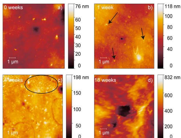
Fig. 2. Topography images, captured using dynamic AFM. The evolution of the surface topography over accelerated weathering time is depicted. (a) Initial state, (b) 1 week accelerated weathering, (c) 4 weeks accelerated weathering, (d) 18 weeks accelerated weathering. Note that the scale is adjusted to every picture so that as many details as possible can be observed. An increase in topological features like round spots (see arrows and marked region) with increasing accelerated weathering time is visible.
