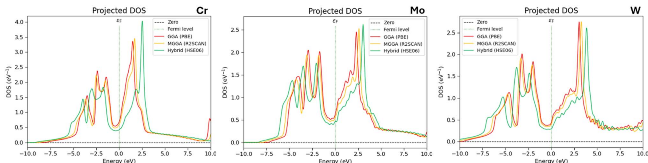
Fig. 1 Comparison of the DOS of chromium (left), molybdenum (center), and tungsten (right). Data obtained with PBE (in red), R 2 SCAN (in yellow), and HSE06 (in green) functionals are compared.
