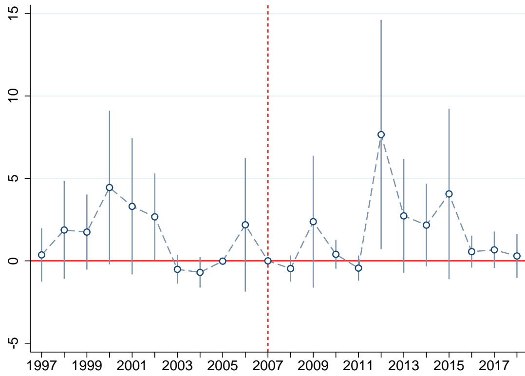
Figure C.1: Event-study analysis of the estimated effect on ethnic conflict
