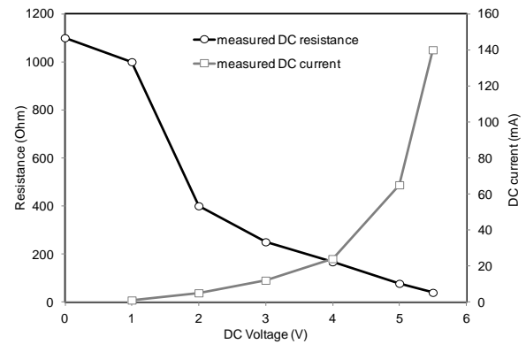
Fig. 7. Measured DC current and DC resistance of the graphene-based microstrip attenuator.
