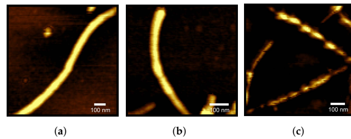
Figure 6. AFM images recorded in Non-contact mode, corresponding to lysozyme fibrillated without taurine (a), with taurine 25 mM (b) and with taurine 400 mM (c).
