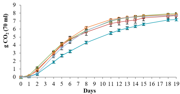
Figure 4. Fermentation kinetics of the new selected strains tested: OKAY (—□—); DiSVA 705 (—△—); I1 (—○—); I4 (—*—); B4 (—+—). The graph represented the fermentation trend in NGJ. The results were the mean values and the standard deviations were represented as error bars.
