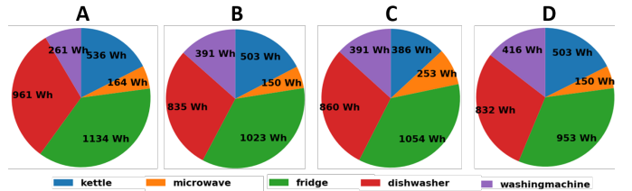
Fig. 6. Energy prediction on UK-DALE data using different models. A: the actual energy; B: the model was trained on REFIT; C: the CNN trained on REFIT was frozen and dense layers were trained on UK-DALE; D: the CNN trained on REFIT using washing machine model was frozen and dense layers were trained on UK-DALE.
