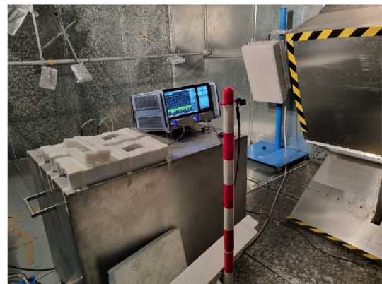
FIGURE 1. Reverberation chamber and the setup used for its characterization.
