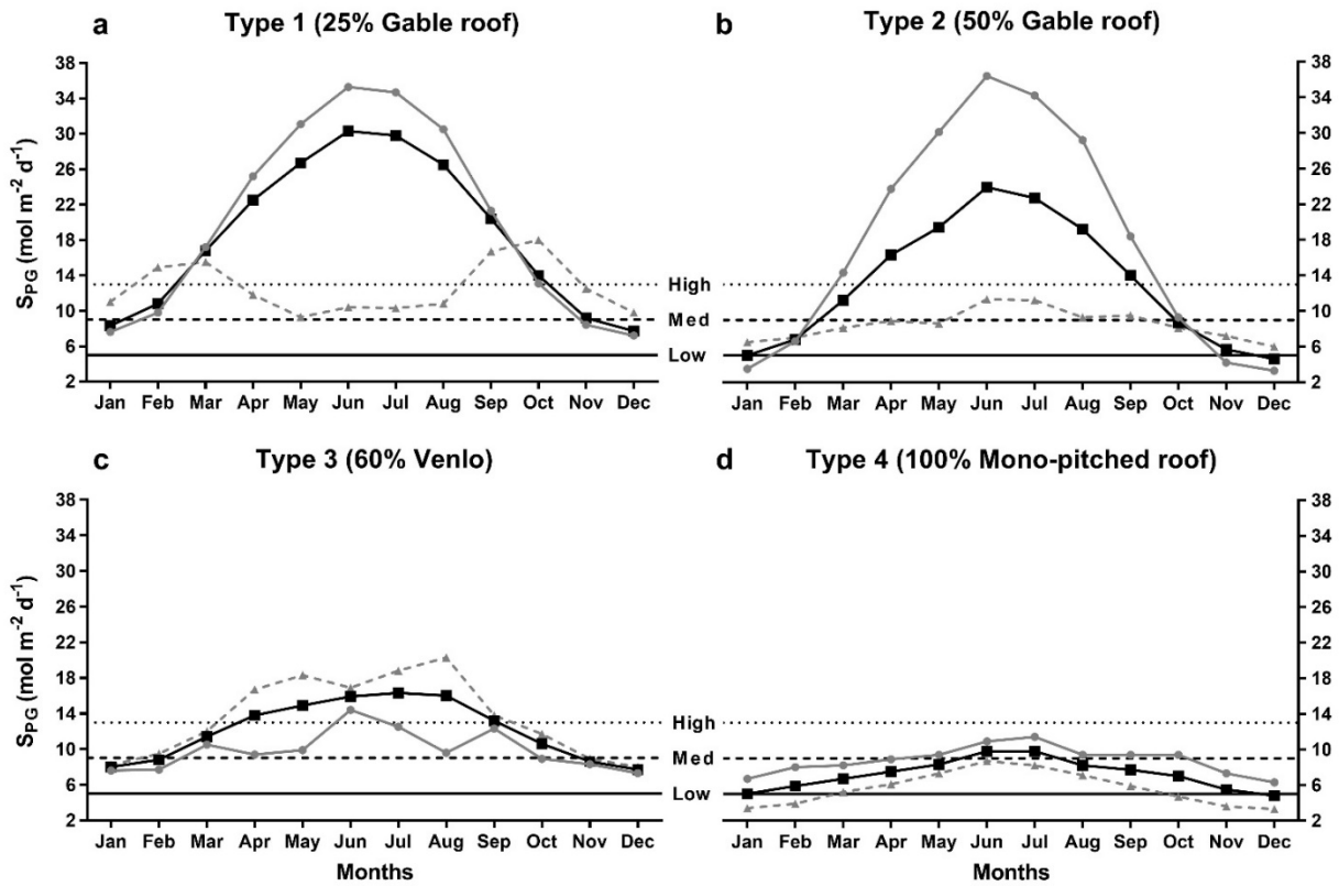
Figure 4. Average monthly SPG inside the four PVG types, compared to the average DLL_{min} requirements of the species considered in the study: high (min. 13 \text{ mol m}^{-2} \text{ d}^{-1} ), medium (min. 9 \text{ mol m}^{-2} \text{ d}^{-1} ) and low light demanding crops (min. 5 \text{ mol m}^{-2} \text{ d}^{-1} ). The average SPG of the whole PVG area is reported (black lines and squares), together with the SPG under the conventional (ST) roof (grey lines and circles) and the photovoltaic (PV) roof (grey dotted lines and triangles). For PVG type 4 ( PV_R 100%), the PV and the ST roof correspond to the N-half and the S-half greenhouse area, respectively.
