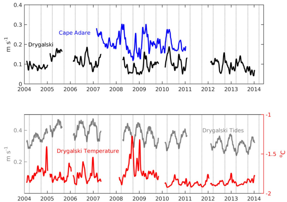
Figure 3. Water properties at Cape Adare and the Drygalski Trough (Top) Monthly-averaged, near-bottom flow at Cape Adare (blue) and in the Drygalski Trough (black) often increase at equinoxes (vertical dotted lines). (Bottom) The tidal flow in the Drygalski Trough, derived by subtracting the subtidal velocities from the full velocities, has a marked variation with lowest tidal flows during equinoxes (vertical lines) and highest tidal flows during solstices. Conservative temperature near bottom in the Drygalski Trough (red) increases during solstice when tidal velocities are highest.
