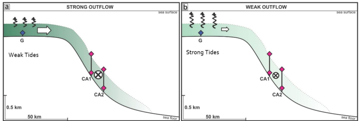
Figure 6. The link between the outflow, the tides and the density in Terra Nova Bay. The flow out of the trough (white arrows) turns to the left and flows along the slope past the moorings (flow is into the page in the diagram and indicated by the circle with a cross). The strength of the outflow depends on the tidal mixing in the trough (curly arrows) and the density of the bottom water from Terra Nova Bay (shown by the green shading where darker green indicates denser water). (a) A stronger outflow of more dense water results when tides are weaker and water in Terra Nova Bay has a higher density. (b) A weaker outflow of less dense water results when tides are stronger and water in Terra Nova Bay is less dense.
