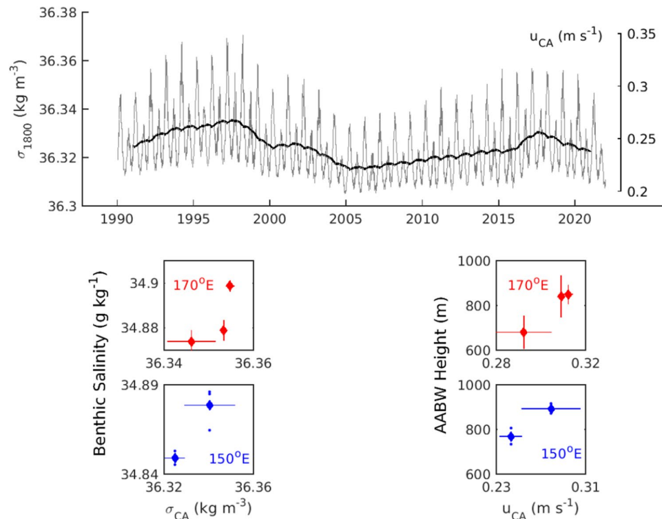
Figure 5. Simulated flow and density of the dense outflow at Cape Adare. (Top) Density and flow at Cape Adare estimated from the tides in the Drygalski Trough and density in Terra Nova Bay. The running average over two years is plotted in black to show the interannual variability. (Bottom left panels) Absolute salinity averaged over the bottom 300 m from hydrography at 170°E (red) and 150°E (blue) is plotted against the estimated outflow density. (Bottom right panels) The height of the 0 °C above bottom in the hydrographic sections at 170°E (red) and 150°E (blue) is plotted against the estimated outflow velocity. See methods for details of the averaging and uncertainty estimates.
