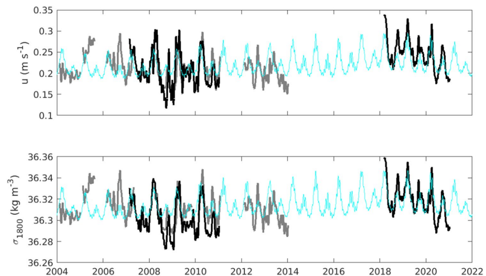
Figure 4. Observed and simulated flow and density at Cape Adare. Flow at the bottom sensor at Cape Adare (top) from measurements at Cape Adare (black lines), inferred values at Cape Adare using observations in the Drygalski Trough (dark gray lines) and simulated velocities at Cape Adare based on tides in the Drygalski Trough and density in Terra Nova Bay (blue line). (Bottom) Density at the Cape Adare mooring from the same set of observations and simulation.
