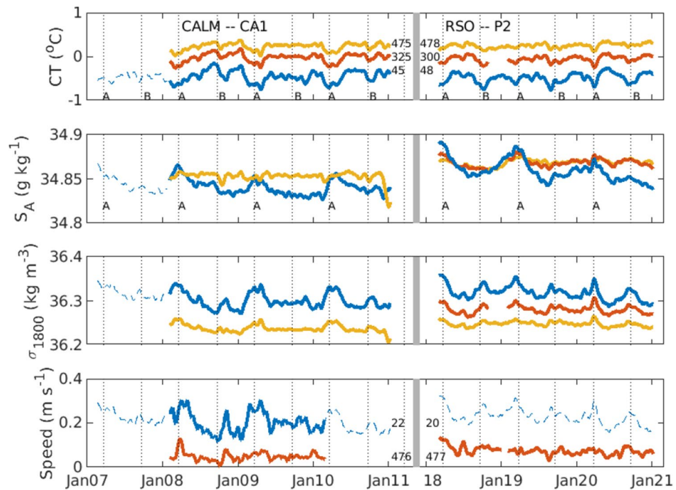
Figure 2. Observations of the dense water outflow at Cape Adare. Conservative temperature, absolute salinity, density referenced to 1800 db, and the flow speed on the slope at 1740 m depth near Cape Adare from sensors on the CA1 and P2 moorings. The height of the sensors above bottom is given by the black numbers in the panels. Dashed lines show a reconstruction of water properties and flow at the lowest sensor from the measurements at the nearby CA2 mooring in 2007 and a reconstruction of the flow from the density at the lowest sensor during the RSO deployments. Tick marks show January of every year with the grey bar indicating a discontinuity in time between the two deployments. Vertical dotted lines indicate the two equinoxes each year.
