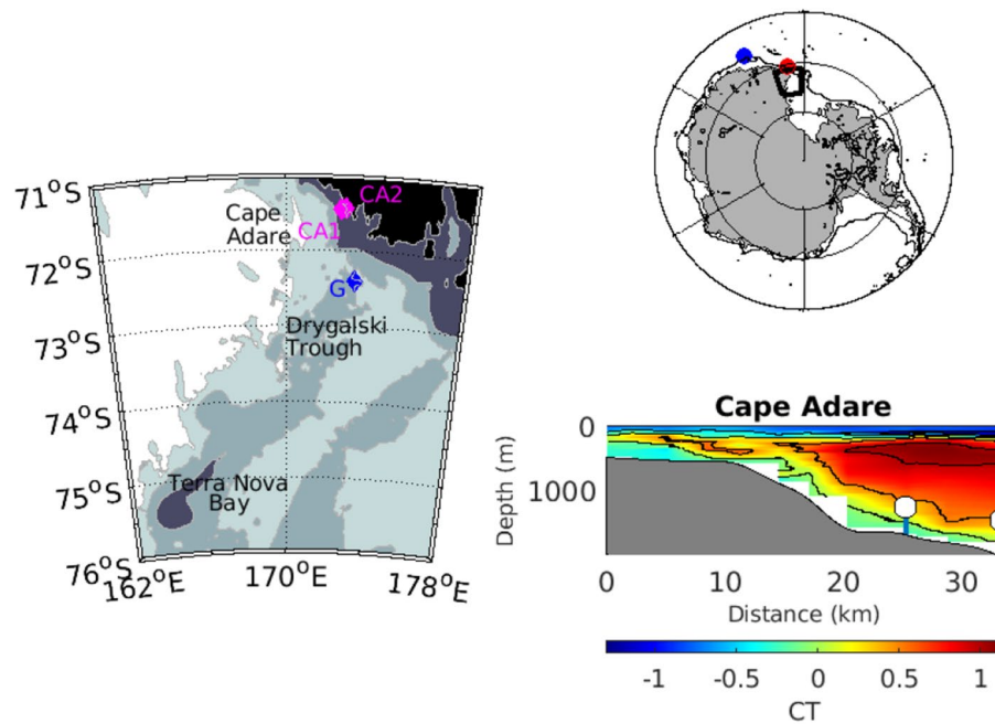
Figure 1. Observations of the dense outflow from the western Ross Sea (Left) Map of the western Ross Sea with the two mooring locations at Cape Adare (CA1/P2 and CA2) indicated by magenta diamonds and Mooring G in the Drygalski Trough indicated by a blue diamond. Depth contours are at 500, 1000 and 2000 m. (Top right) Outline of the western Ross Sea map inset is shown in black with the locations of the hydrographic observations at 170°E indicated by the red circle and 150°E by the blue circle. (Bottom right) The positions of the two moorings at Cape Adare (CA1 and P2 at the shallower depth; CA2 at the deeper depth) measuring benthic flow on the slope are shown with conservative temperature from the 2018 hydrographic section.
