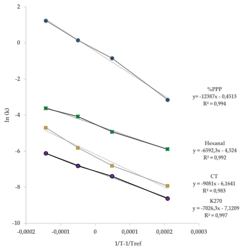
Figure 3. Arrhenius plot of apparent zero-order rate constants of K270, CT and %PPP.
