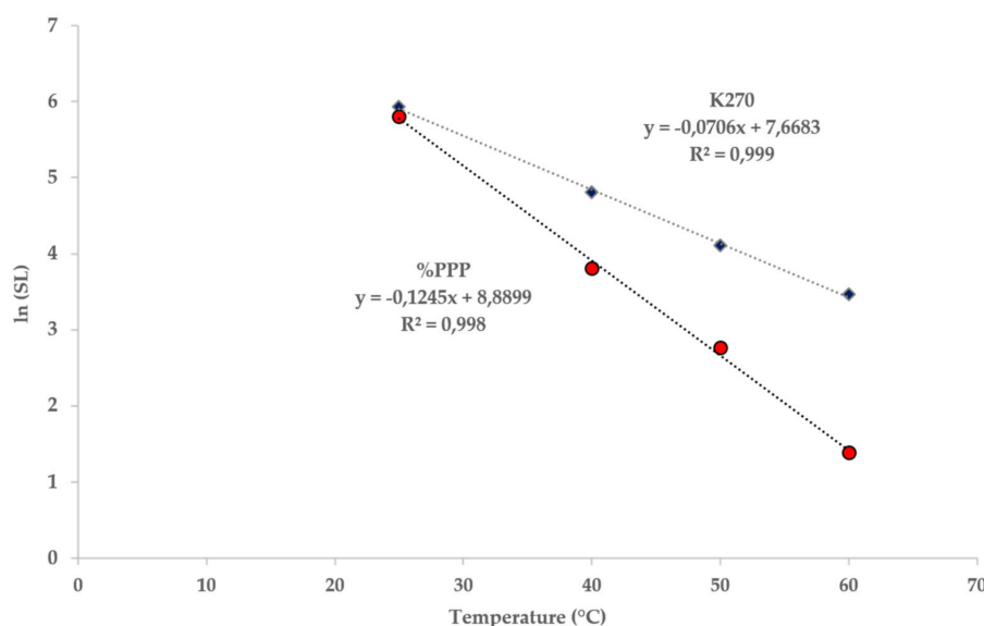
Figure 4. Shelf-life plots of EVOO by using K270 and %PPP as shelf-life indicators.
