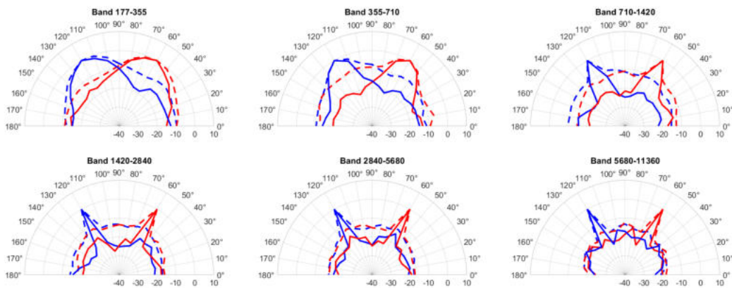
Figure 5: Directivity patterns obtained with IRs measured in the semi-anechoic chamber pointing at 60° (blue curve) and at 120° (red curve), before (dashed curve) and after applying the side lobes reduction (solid curve).
