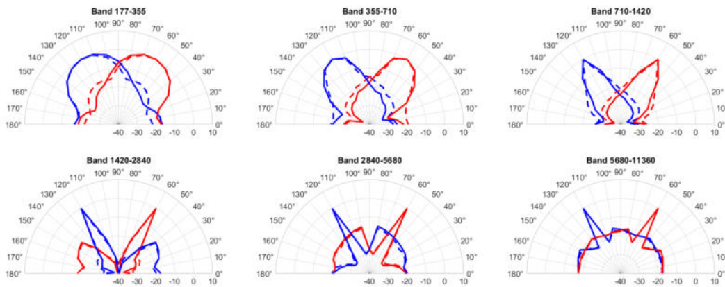
Figure 2: Directivity patterns obtained with simulated IRs pointing at 60^\circ (blue curve) and at 120^\circ (red curve), before (dashed curve) and after applying the side lobes reduction (solid curve).
