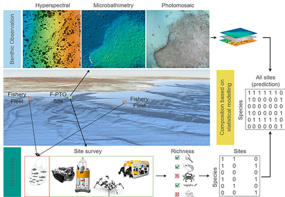
Fig. 9. Site-specific ecological knowledge obtained via multiparametric monitoring, which is spatially scaled for predictions of species distributions and abundances. The presence and abundance of benthic species can be tracked over time at any monitored and mapped site (by F-PTOs, via the combination of different imaging approaches). The results can be compared with similar data from nearby areas (e.g., fishery-dependent trawl data, with commercial vessels being a part of the G-PTO framework). Predictions of species presence and abundance can then be formulated for any other non-surveyed area for which only seascape data are available.
