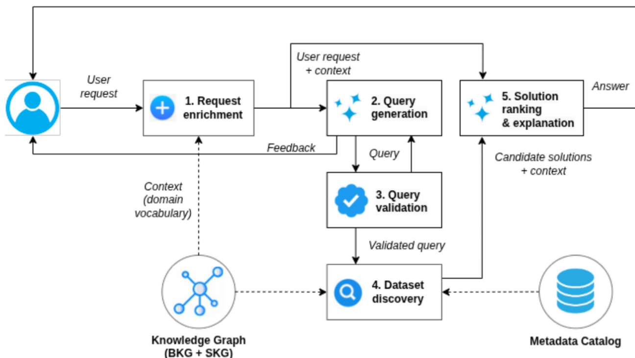
Fig. 3 Architecture of the Graph RAG approach
