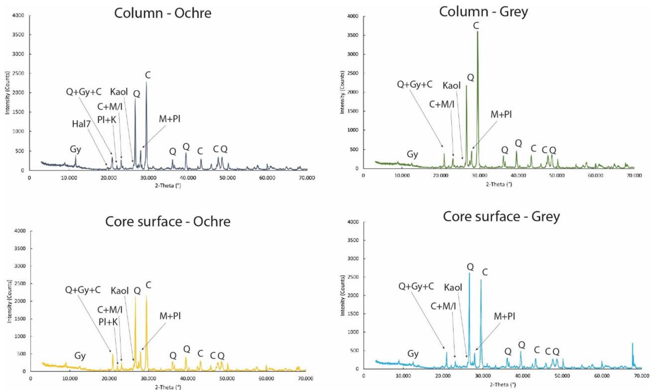
Fig. 15 XRD spectra of the column and core samples for the ochre and grey zones highlight similar mineralogic composition for all four samples: C, calcite; Q, quartz; Pl, plagioclase; Gy, gypsum; Hal7, halloysite-7Å; Kaol, kaolinite; M/I, muscovite/illite
