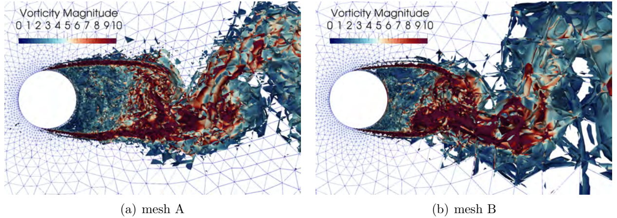
Figure 9: Flow around a circular cylinder - Mesh details and instantaneous isosurfaces of the Q-criterium coloured with the vorticity magnitude
