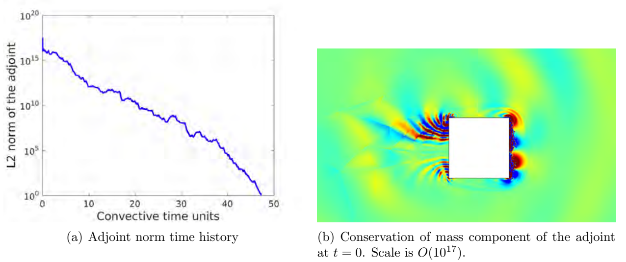
Figure 4: Flow around a square - Growth of the adjoint for the time-averaged drag output in reverse time
