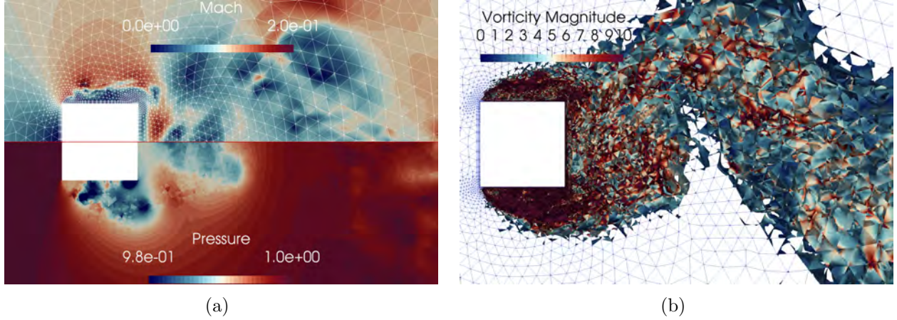
Figure 16: Flow around a square cylinder - Instantaneous Mach number and pressure contours (a), and isosurfaces of the Q-criterion coloured with the vorticity magnitude contours (b)
