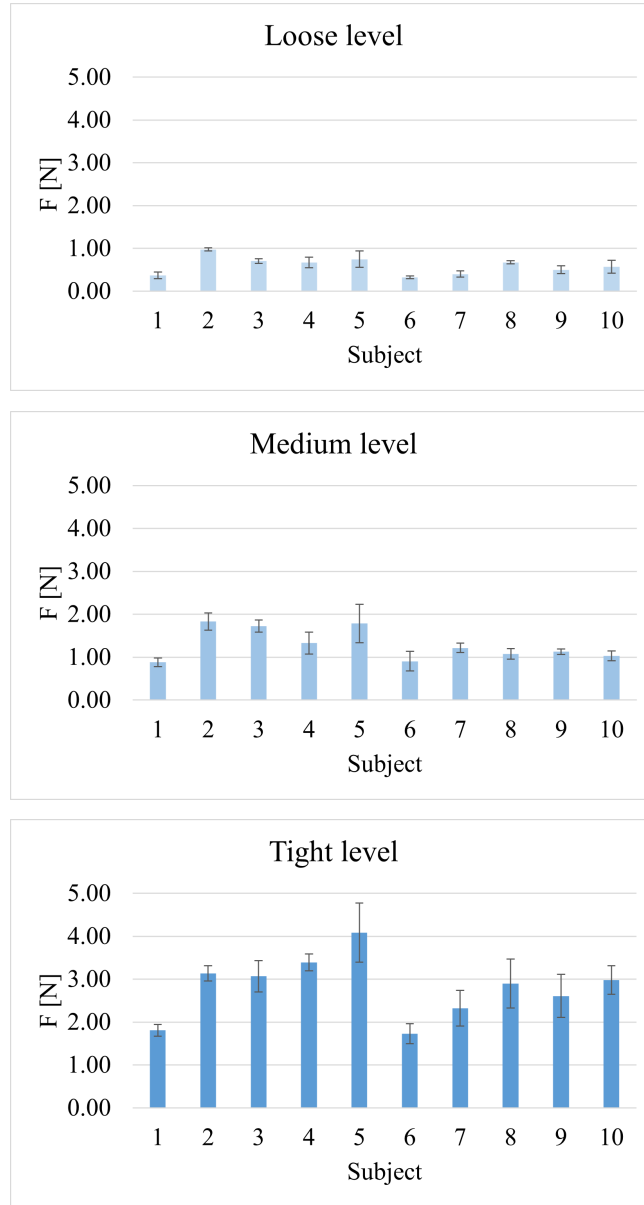
Fig. 5. Tightening force intervals (mean±standard deviation) measured for loose (top), medium (centre) and tight (bottom) levels, for the whole population.
