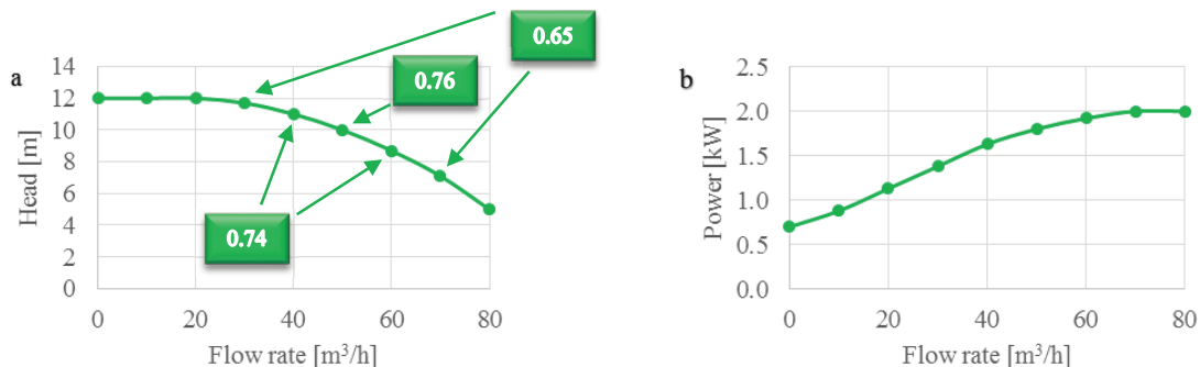
Fig. 4. (a) Characteristic curve of the selected pump; (b) Power curve of the selected pump
