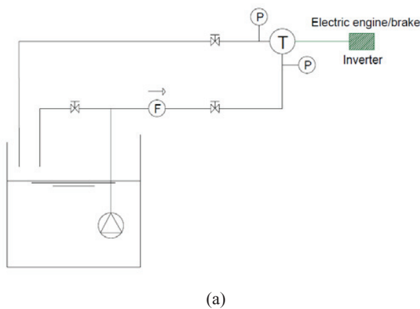
Fig. 2. Sketch of the test bench (a) and the real test bench (b) used for performing tests on the selected pump in turbine mode
