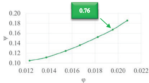
Fig. 6. Non-dimensional characteristic curve of the selected pump running in reverse mode
