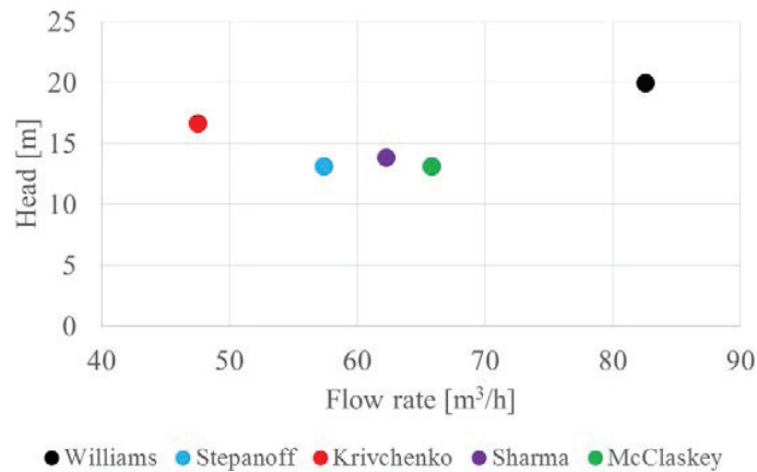
Fig. 1. Scenario of possible BEP values achieved by the selected pump
