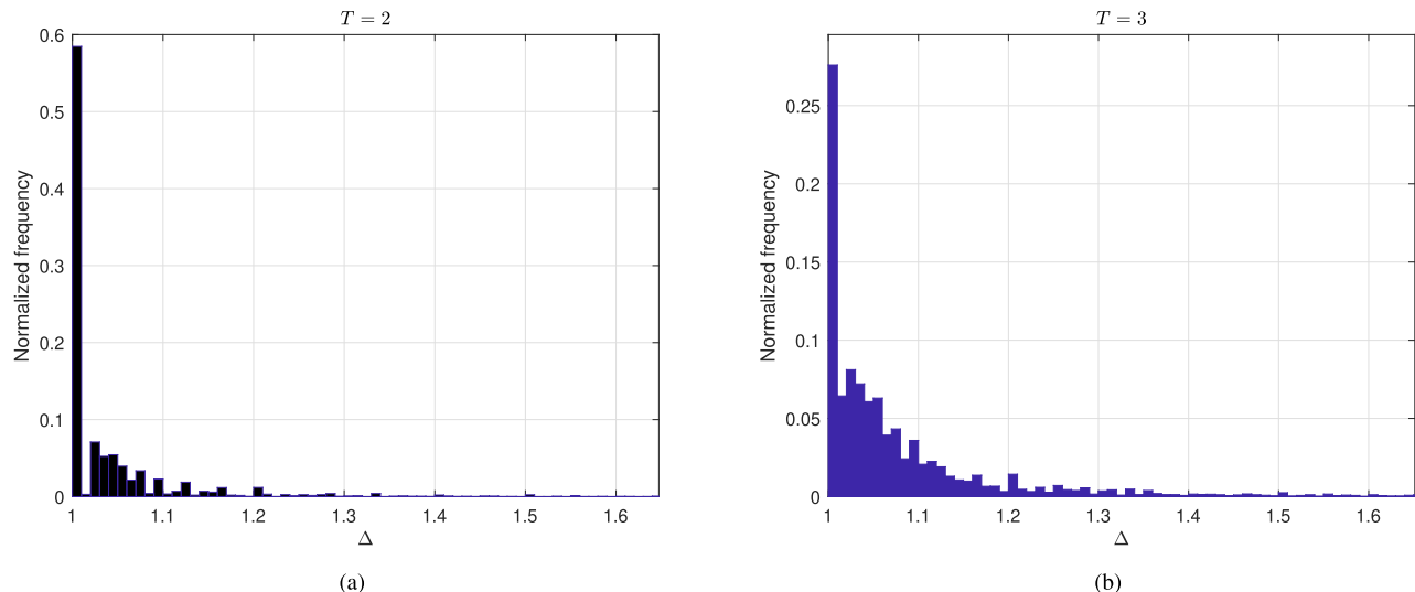
Fig. 3. Normalized frequency of the ratio between d_{\mathcal{E},T} and d_{\mathcal{C},T} , for 10 000 PTV-SC-LDPC codes with (a) T = 2 and (b) T = 3 .
