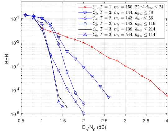
Fig. 4. Bit error rate vs signal-to-noise ratio, for codes with different period and memory.
