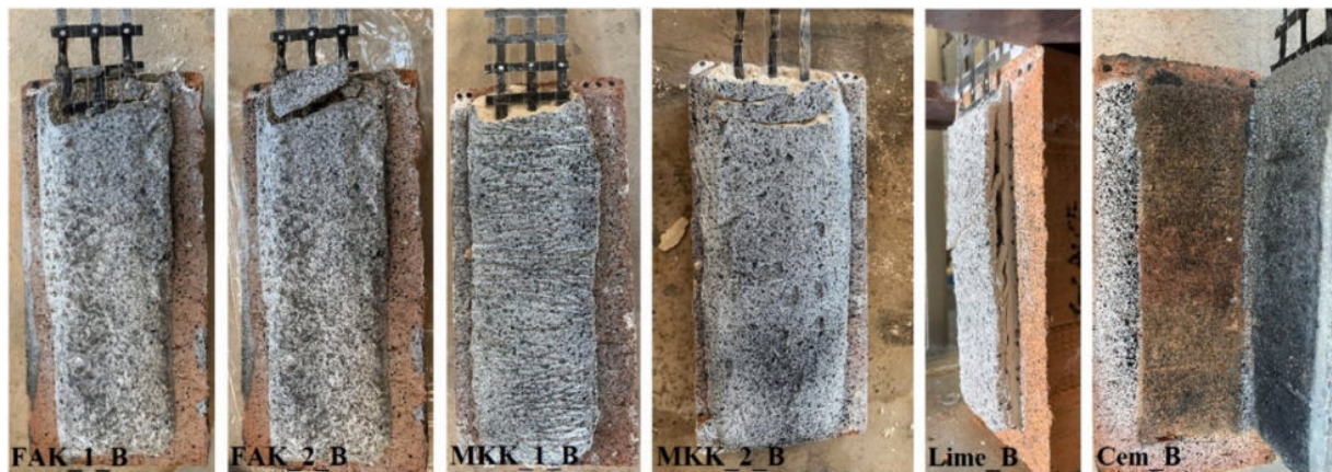
Fig. 11. Failure modes observed in shear bond tests.
