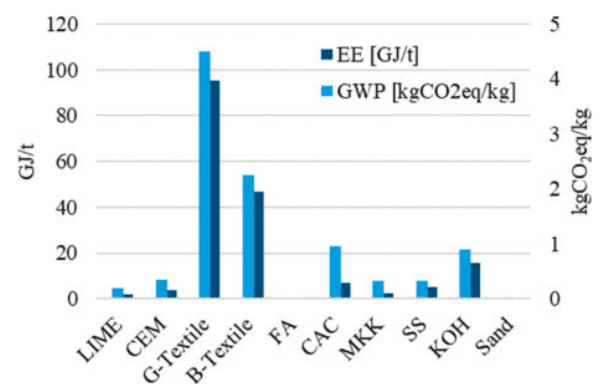
Fig. 5. Required energy and GHG emissions of TRM constituent materials.
