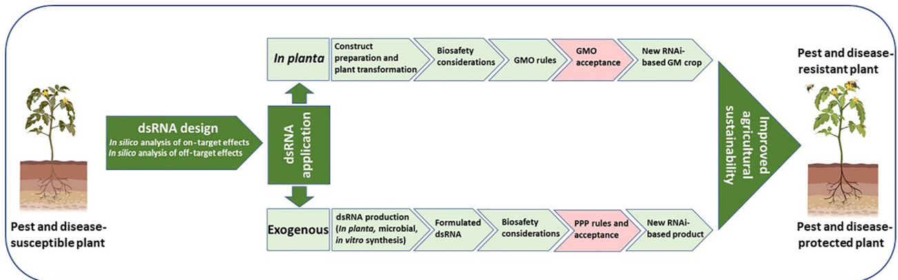
Figure 2. Two Main Delivery Approaches for RNAi-Based Control of Pests and Diseases. RNAi-based control typically starts with designing the double-stranded (ds)RNA active molecule to be specific to an essential gene in the pest or pathogen, while remaining safe for non-target organisms. The increase in availability of genome/transcriptome databases for more organisms and the development of sophisticated high-throughput approaches, such as RNA-seq and digital gene expression tag profile (DGE-tag) technologies, has significantly improved the selection of potential RNAi targets. Although in silico tools can help in the design of pest or pathogen-specific dsRNA molecules, empirical evidence from bioassays is required to support effectiveness against the pest/pathogen and zero to negligible adverse effects in non-target organisms. There are two main dsRNA application approaches for RNAi-based control; one approach involves the in planta expression of RNAi constructs to target genes of pests/pathogens, while the second approach involves the exogenous application of dsRNA. The choice of the application method depends on the interaction between the crop and the pest/pathogen, and on the feasibility of developing an efficient application method against the pest/pathogen. These delivery approaches follow two separate paths during the product development pipeline, with the in planta approach falling under genetically modified organism (GMO) regulation, while the exogenous approach is expected to fall under the plant protection product (PPP) regulation. The genetically modified (GM) approach can be challenged by a lack of technological tools to modify some plant species, high cost of production to registration of the GMO, and some public opposition to GMOs. The exogenous approach is challenged by the high cost of producing dsRNA for large-scale field application and the lack of appropriate formulation technologies to improve RNAi efficiency against recalcitrant pests/pathogens. Despite these challenges, both delivery approaches have successfully led to the development of safe and effective RNAi-based products, which can significantly contribute to agricultural sustainability by reducing the use of contentious pesticides.
