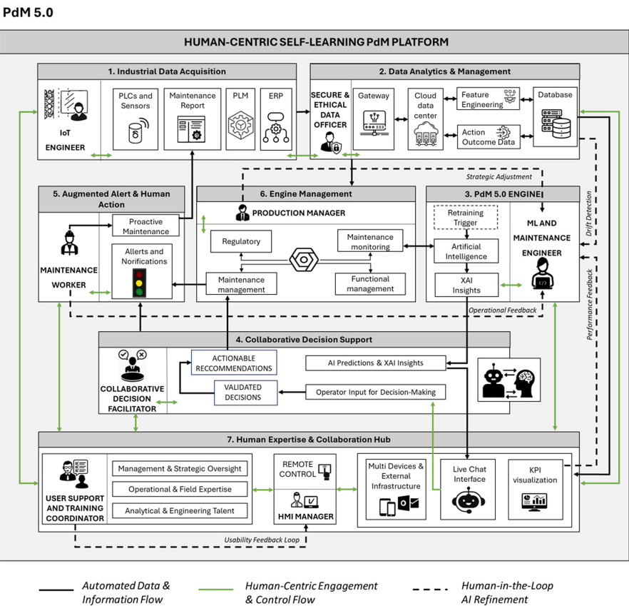
Figure 1. Architecture of the PdM 5.0 platform
