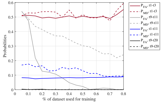
(b) CFR with an LSTM network
