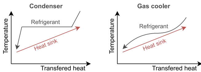
Fig. 1. Temperature profile during heat rejection for subcritical operation (condenser) and transcritical or supercritical operation (gas cooler).
