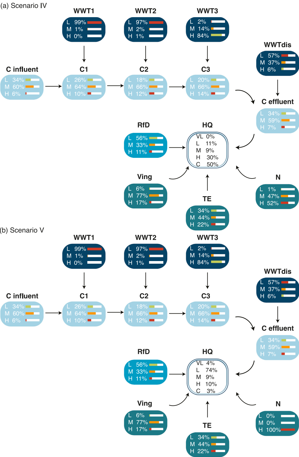
Fig. 9. Estimated hazard quotient (HQ) under (a) unintended ingestion of water by agricultural workers during crop harvesting (Scenario IV), (b) reduced exposure due to the use of personal protective equipment (PPE) (Scenario V).
