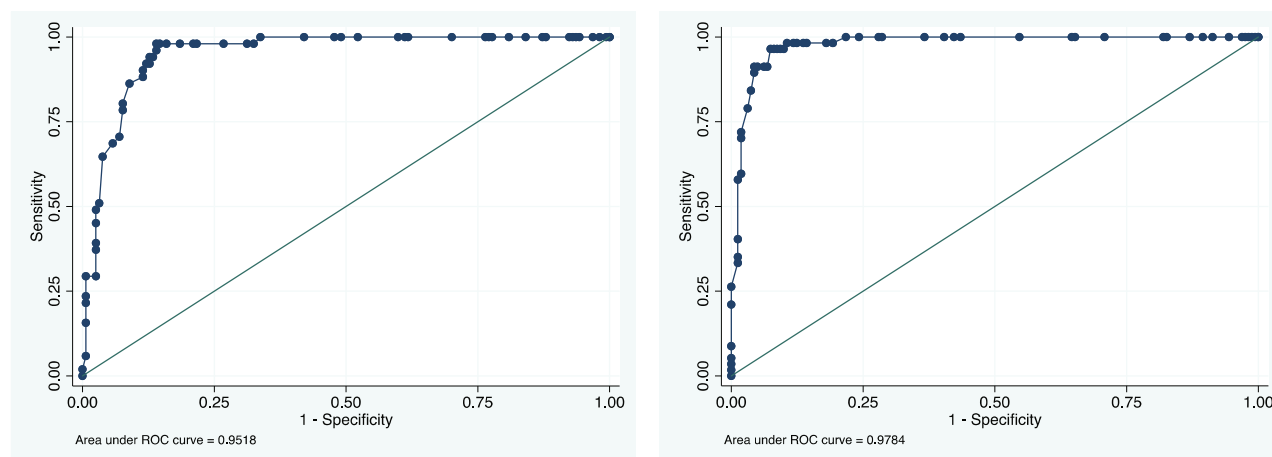
Figure 4. Receiver operating characteristic (ROC) curves in the derivation cohort (left) and validation cohort (right) for the patients who were eligible to be scored for classification of CPPD disease. In the derivation cohort, data for 60 definite cases and 148 definite mimickers were included. In the validation cohort, data for 65 definite cases and 162 definite mimickers were included. Color figure can be viewed in the online issue, which is available at http://onlinelibrary.wiley.com/doi/10.1002/art.42619/abstract .
