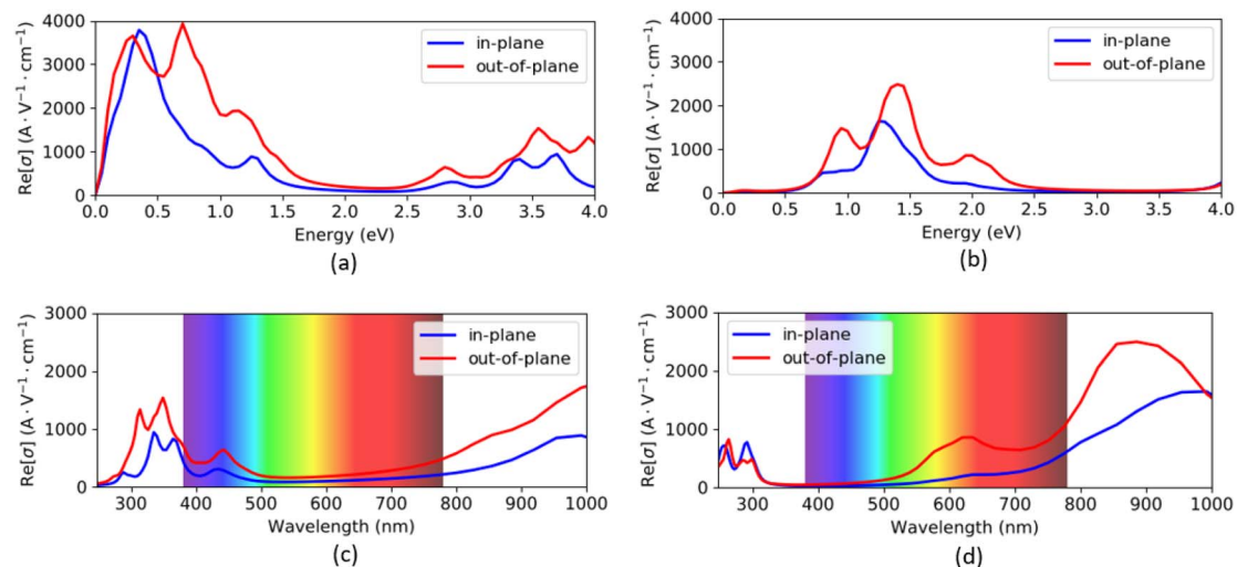
Fig. 6 Optical conductivity as functions of energy and wavelength of \text{VO}_2(\text{B}) polymorph along with in-plane and out-of-plane directions predicted by PBEsol (a and c) and PBEsol/HSE (b and d), respectively.
