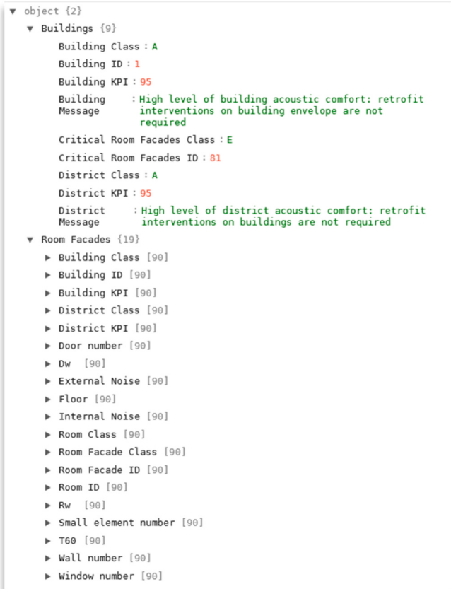
Fig. 8. Result obtained for “acoustic_calculation” in JSON format.
