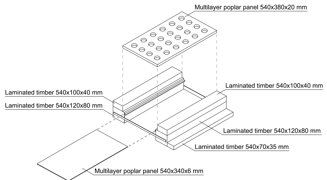
Figure 5. Details of the NSD base.
