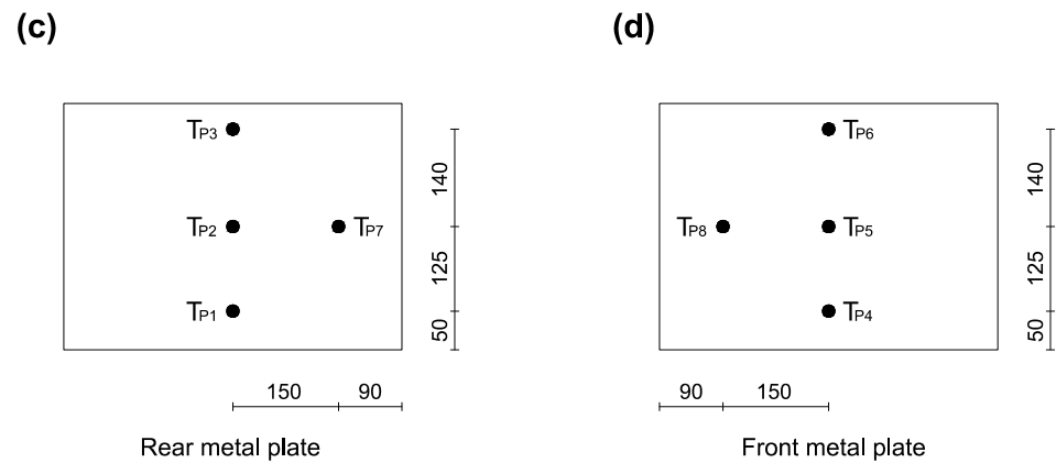
Figure 10. Position of the thermocouples for the 17 February 2023 test: (a) in the central area of the drying chamber; (b) in the lateral area of the drying chamber; (c) on the rear metal plate; (d) on the front metal plate. The dimensions are in mm. The thermocouple supports and the glass plates are highlighted in red and blue, respectively.
