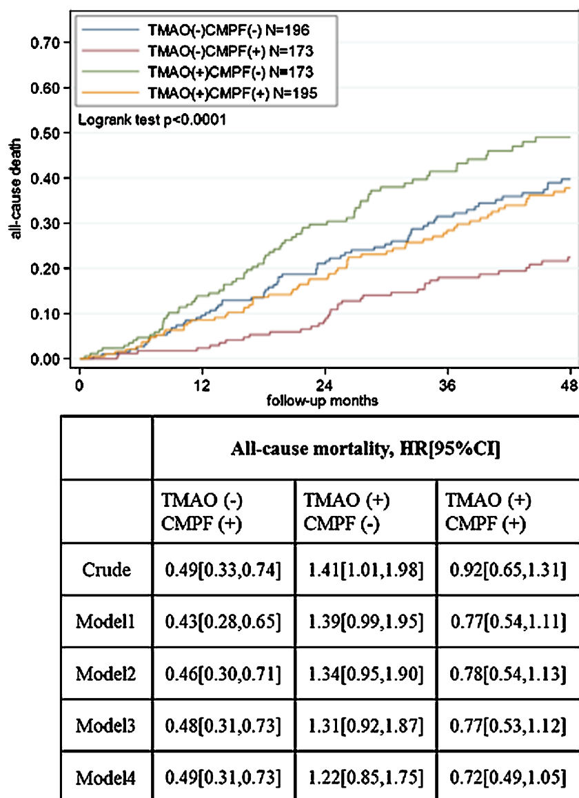
FIGURE 1 Kaplan–Meier estimates for all-cause mortality and cause-specific Cox regression models according to TMAO and CMPF median groups. Model 1 adjusted for age, sex, country. Model 2: adjusted as for model 1 plus diabetes, preexisting cardiovascular disease, Charlson comorbidity index, diastolic blood pressure, systolic blood pressure, malnutrition (SGA <5). Model 3: adjusted as for model 2 plus albumin, phosphate, hemoglobin. Model 4: adjusted as for model 3 plus eGFR. CMPF, 3-carboxy-4-methyl-5-propyl-2-furanpropionate; eGFR, estimated glomerular filtration rate; SGA, subjective global assessment; TMAO, trimethylamine N-oxide.
