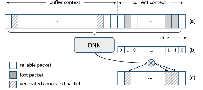
Fig. 1. Overview of the proposed adaptive latency PLC mechanism, operating on a given audio segment. The current context (a) can be varied between 1 and 51 packets during inference, by modifying the buffer length accordingly. (b) represents the binary mask denoting lost (1) and reliable (0) packets, based on which the repaired current context (c) is rearranged.
