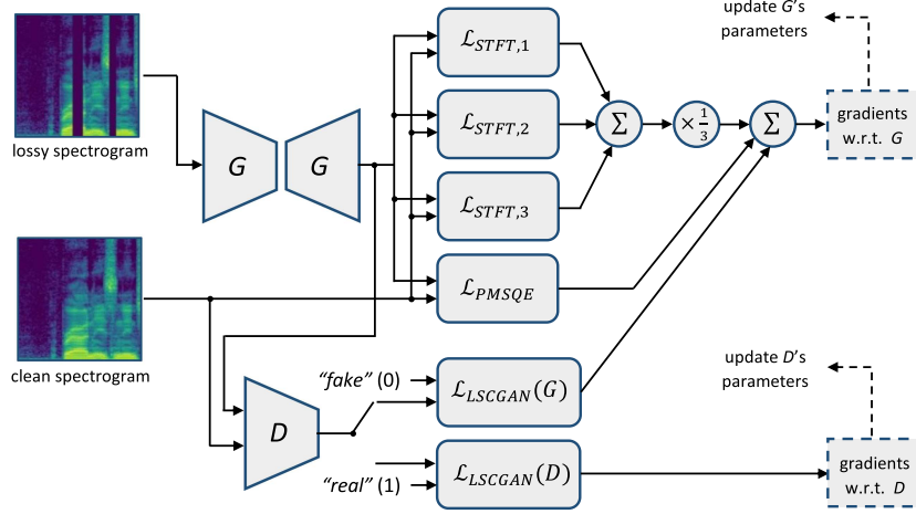
Fig. 3. Illustration of the adversarial training strategy, assisted by the losses: \mathcal{L}_{LSCGAN}(G) of (2), \mathcal{L}_{LSCGAN}(D) of (3), the multi-resolution STFT loss of (4) and the perceptual loss \mathcal{L}_{PMSQE} of (9).
