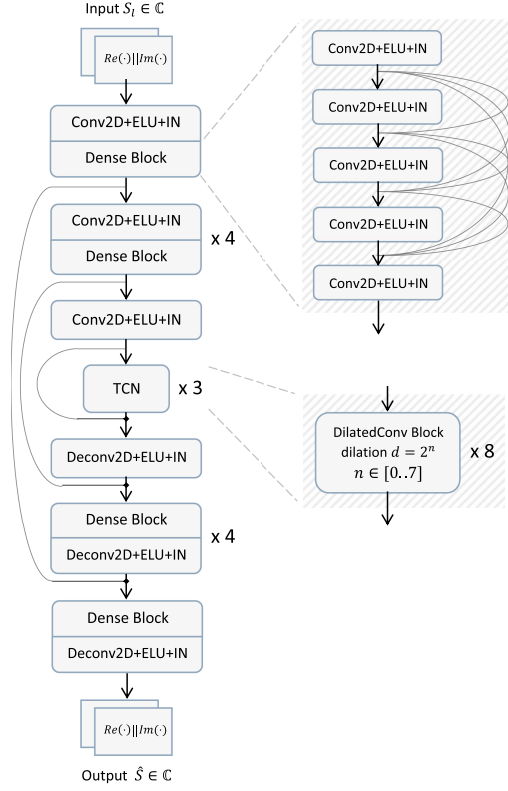
Fig. 2. Generator network composed of the U-Net with temporal convolutional (TCN) bottleneck. As input to the generator is the complex-valued lossy spectrogram S_l , which is processed as a 2-channel feature map, consisting of the real and imaginary part of S_l . The network outputs the repaired spectrogram \hat{S} having the same size as the input.
