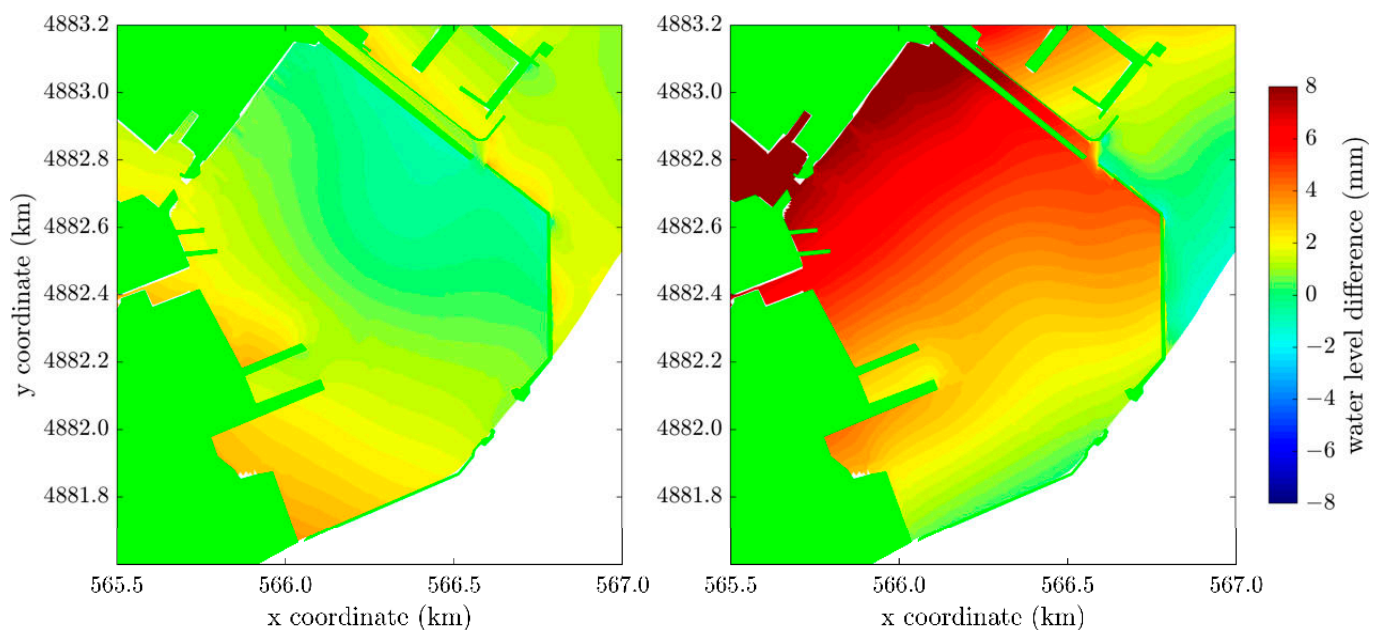
Figure 15. Water level differences between the cases with NNE wind and no wind ((left) panel) and the cases with SSE wind and no wind ((right) panel).
