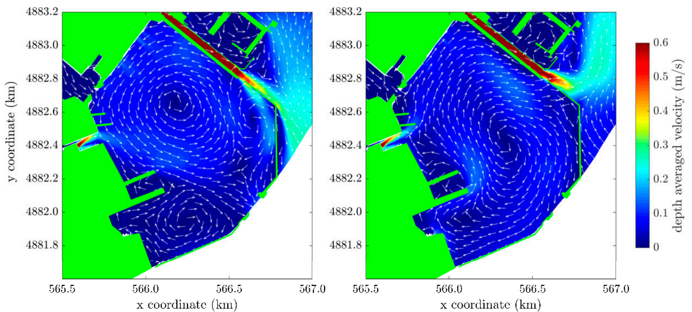
Figure 7. Modelled hydrodynamic circulation under NNE wind ((left) panel) and SSE wind ((right) panel) at the peak of the rivers' discharges for the TR scenario. The arrows only indicate the velocities' direction, while the intensity is given by the colormap.
