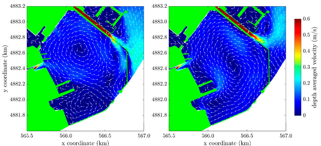
Figure 10. Modelled hydrodynamic circulation under NNE wind ((left) panel) and SSE wind ((right) panel) at the peak of the rivers' discharges for the TWR scenario. The arrows only indicate the velocities' direction, while the intensity is given by the colormap.
