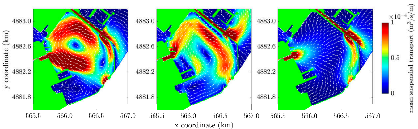
Figure 14. Mean suspended sediment transport for the TR scenario in case of NNE wind ((first) panel), SSE wind ((second) panel), and no wind ((third) panel). The intensity is given by the colour bar, while the direction is represented by the arrows.
