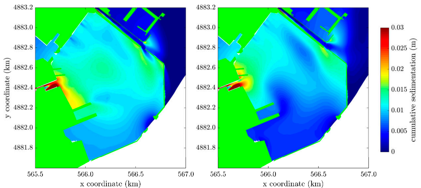
Figure 9. Modelled sedimentation patterns for NNE ((left) panel) and SSE ((right) panel) winds for the TR scenario.
