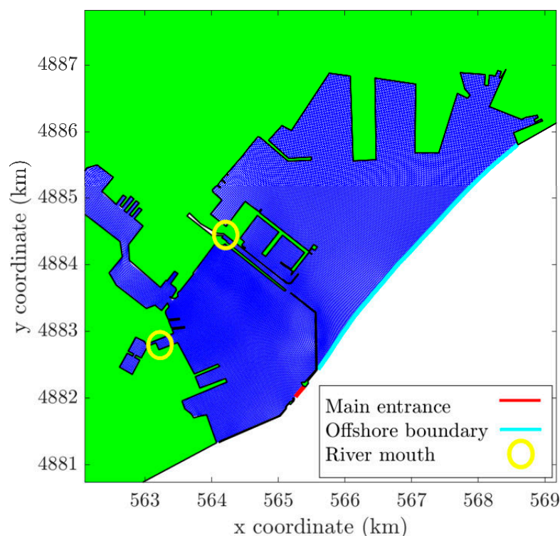
Figure 4. The computational domain of the Arsenale and shipping areas, used for the Delft3D simulations.
