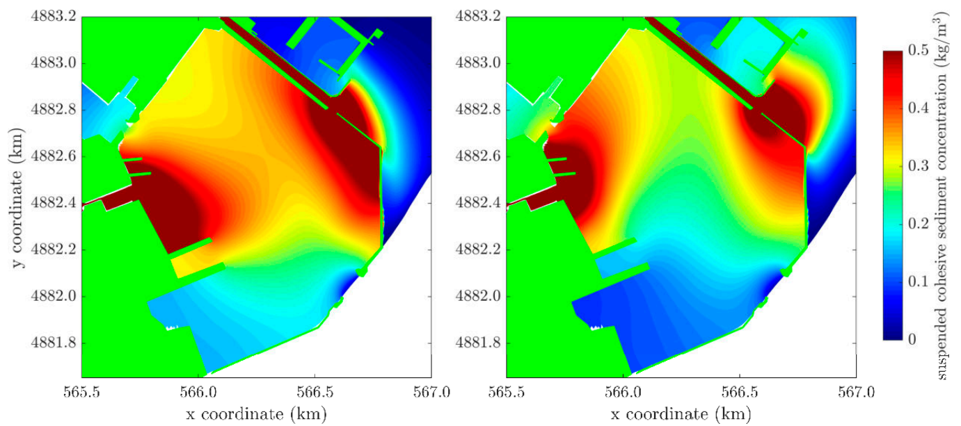
Figure 11. Modelled suspended sediment concentration for NNE ((left) panel) and SSE ((right) panel) winds at the peak of the rivers' discharges for the TWR scenario.
