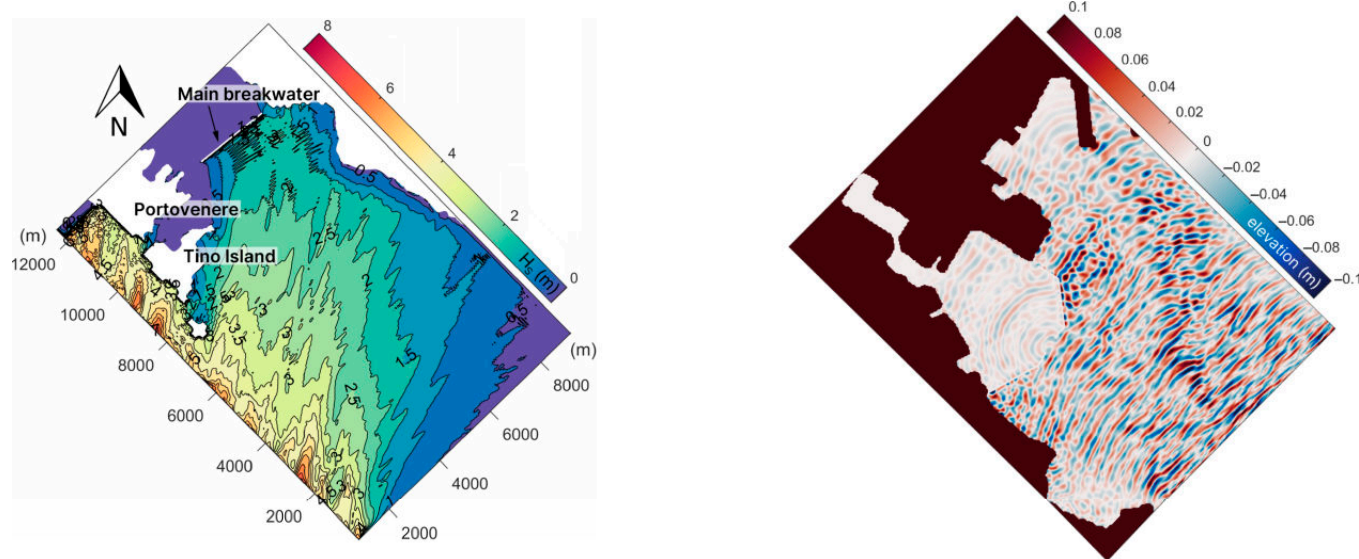
Figure 5. Wave propagation in the outer FUNWAVE model ((left) panel); water elevation in the inner FUNWAVE model ((right) panel).
