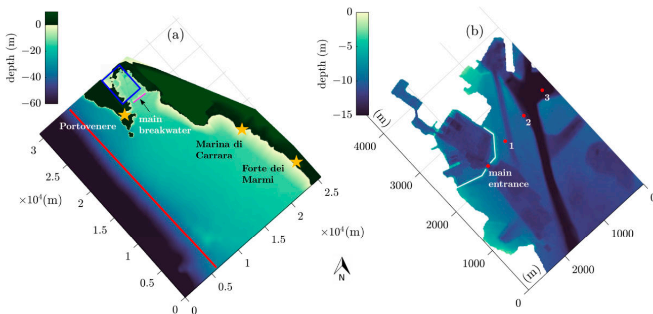
Figure 3. (a) Outer FUNWAVE domain; the red line represents the boundary where the waves were imposed; the blue rectangle highlights the inner domain shown in panel (b). The red dots represent the probes at which local modelled wave time series were extracted.
