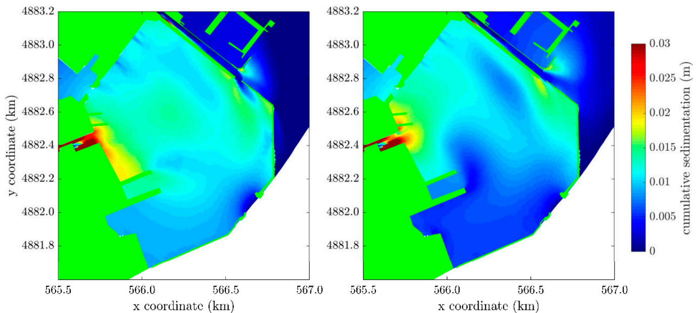
Figure 12. Modelled sedimentation patterns for NNE ((left) panel) and SSE ((right) panel) winds for the TWR scenario.
