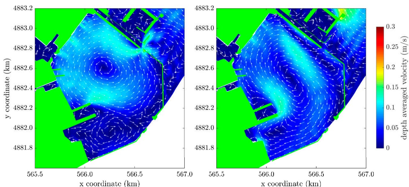
Figure 6. Modelled hydrodynamic circulation forced by NNE wind ((left) panel) and SSE wind ((right) panel). The arrows give the velocity direction, while the intensity is given by the colormap.
