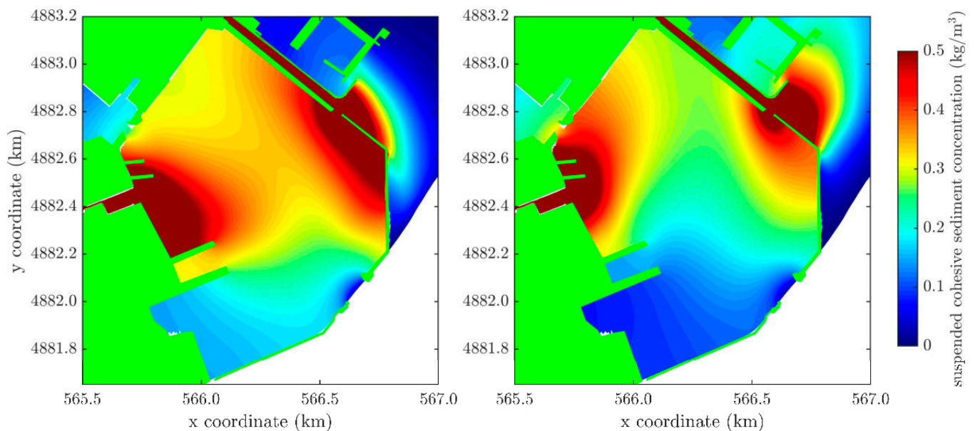
Figure 8. Modelled suspended sediment concentration for NNE ((left) panel) and SSE ((right) panel) winds at the peak of the rivers' discharges for the TR scenario.
