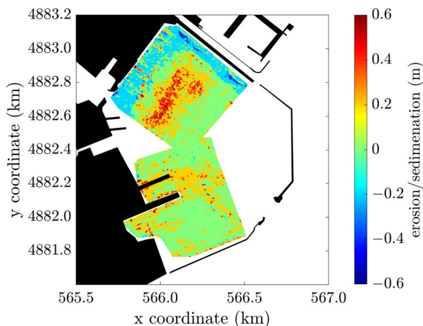
Figure 17. Difference between the surveys performed within the Arsenale in 2013 and 2016. Negative and positive values represent erosion and deposition, respectively.
