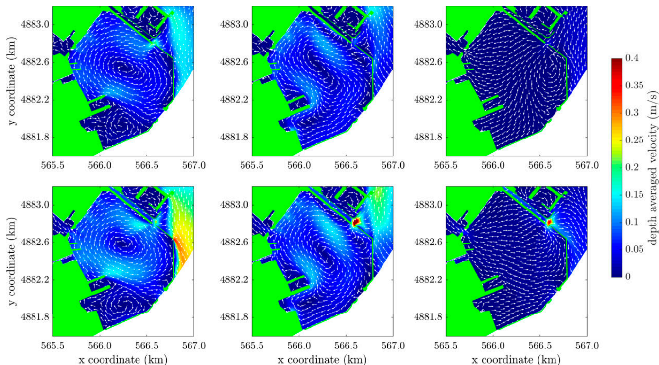
Figure 13. Modelled depth-averaged velocities for NNE wind ((first) column), SSE wind ((second) column), and no wind ((third) column) at tidal filling ((top) row) and emptying ((bottom) row).
