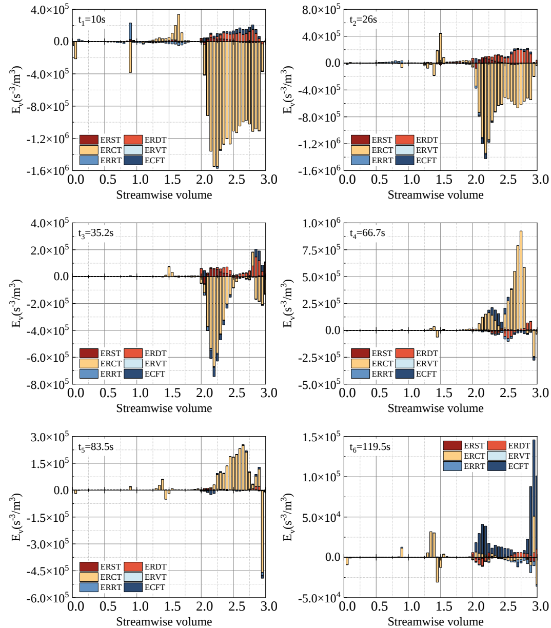
Figure 11. The distribution and intensity of E_v variation along the streamwise direction
