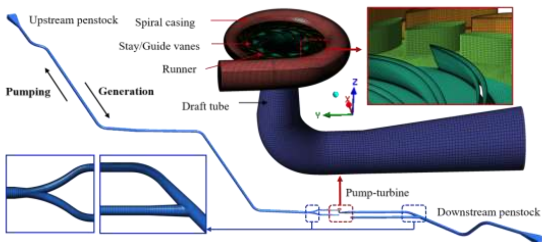
Figure 1. Computational domain and grid of the pumped storage power station
