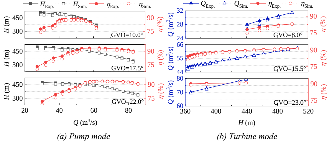
Figure 2. Experimental vs. numerical results of the pump-turbine performance in both pump and turbine modes
