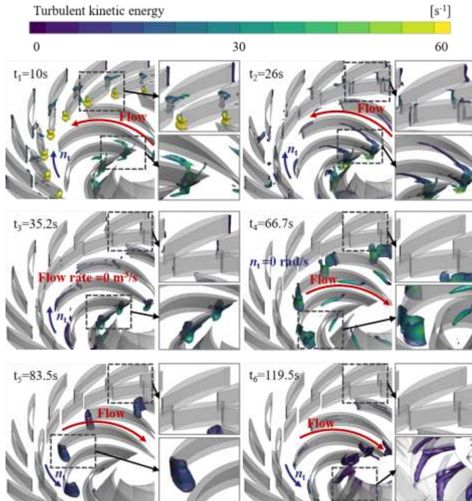
Figure 8. Vortical structures during the fast pump-to-turbine transition process (Rigid vorticity = 120 \text{ s}^{-1} , colored by turbulent kinetic energy)
