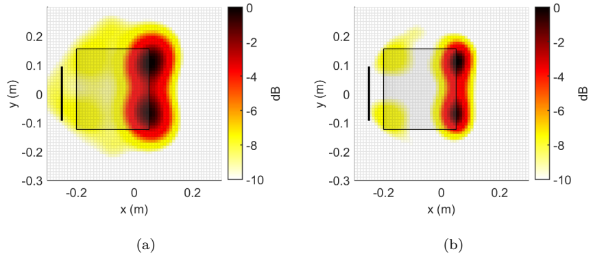
Figure 20: Acoustic maps of airfoil for 2.5 kHz one-third octave band, corresponding to He = [8.4 - 10.5] . (a) CB (b) OC-FB.
