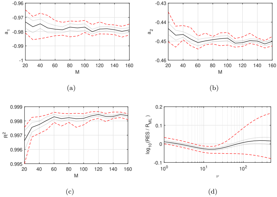
Figure 9: Statistics of fitting parameters. Microphone number range: M = 20\text{--}160 . Vogel spiral parameter range: V = 0.1\text{--}5 . Frequency range: He = 4\text{--}32 , i.e. Hz = 0.125\text{--}1 . Order range \nu = 1\text{--}500 . Black solid line: average values. Grey solid line: average \pm one standard deviation. Red dashed line: maximum and minimum values. (a) a_1 . (b) a_2 . (c) R^2 (d) Fitting residuals. Relative values are calculated with respect to R_{ML} provided by the linear model.
