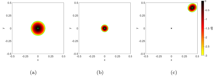
Figure 6: Visualization of CB mainlobe and measured MLW. Green dotted lines is the mainlobe circumference and green cross is the source location. (a) Example 1: on-axis source at He = 4 ( R_{\text{ML}} = 0.140 ). (b) Example 2: on-axis source at He = 8 ( R_{\text{ML}} = 0.070 ). (c) Example 3: off-axis source at He = 8 ( R_{\text{ML}} = 0.085 ), black cross is the array axis.
