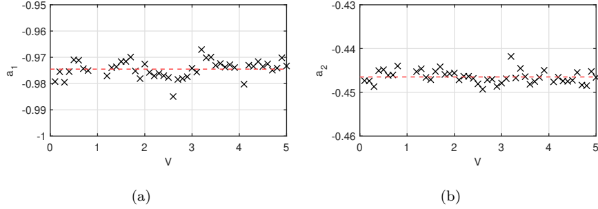
Figure 8: Trend coefficients of MLW for different array design ( M = 40 ) where the V parameter of the Vogel spiral is changed;. Frequency range: He = 4-32 , i.e. He = 0.125-1 . Order range \nu = 1-500 . (a) a_1 . (b) a_2 .
