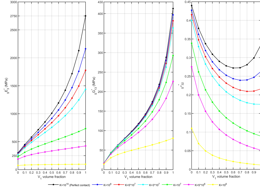
Fig. 2: Effective engineering moduli ( {}_sE_3^* , {}_sG_{13}^* , and {}_sv_{32}^* ) related to stiffness versus V_1 volume fraction of a bi-laminated Cosserat composite with uniform imperfect contact conditions.
