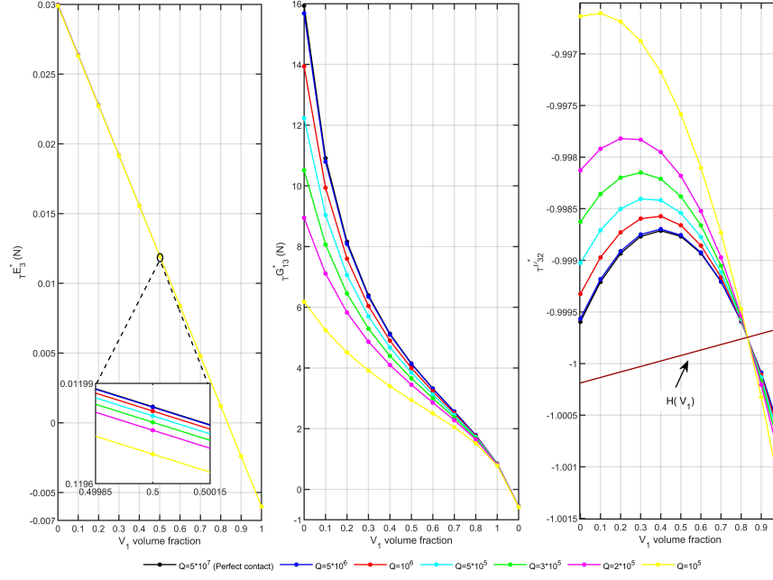
Fig. 3: Effective engineering moduli ( {}_tE_3^* , {}_tG_{13}^* , and {}_t\nu_{32}^* ) related to torque versus V_1 volume fraction of a bi-laminated Cosserat composite with uniform imperfect contact conditions.
