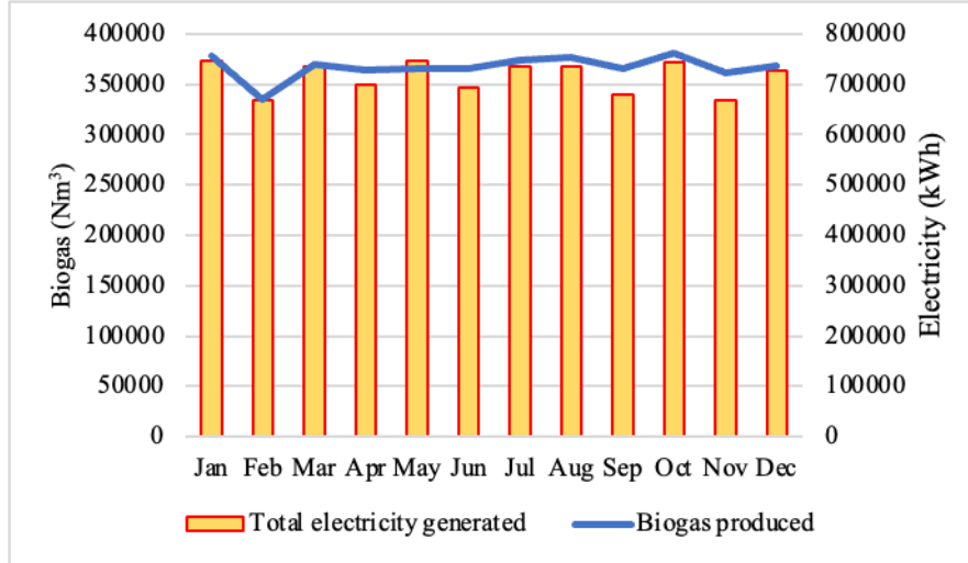
Fig. 2. Monthly biogas produced vs electricity generated.
