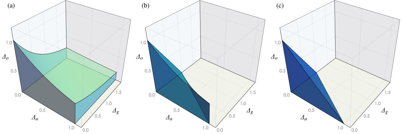
Figure 4: Three-dimensional domains of spectral compatibility in the bandwidth space \mathcal{A} = \{\Delta_a, \Delta_g, \Delta_o\} : (a) domain \mathcal{B}_A compatible with Criterion A , (b) domain \mathcal{B}_B compatible with Criterion B , (c) domain \mathcal{B}_C compatible with Criterion C .
