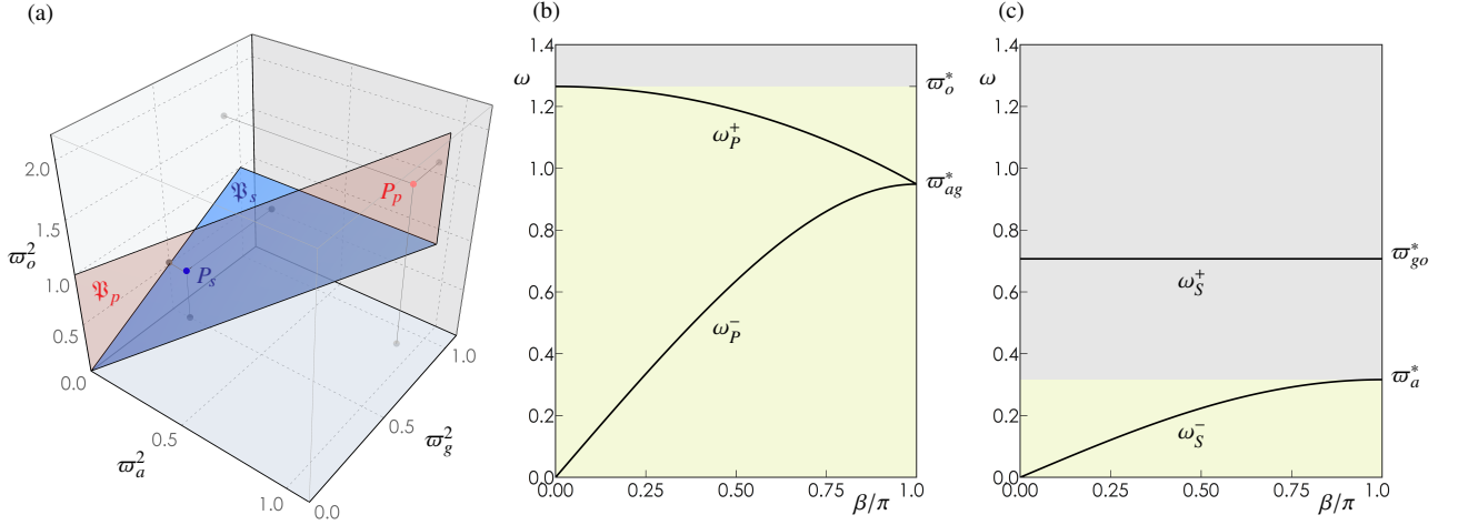
Figure 7: Design of extreme metamaterials: (a) compatible surfaces \Psi_p (red) and \Psi_s (blue) in the three-dimensional space \mathbb{B}^2 of band structures; (b) dispersion spectrum of the superpropagator \mathcal{M}_p^p (red point P_p on \Psi_p ), (c) dispersion spectrum of the superfilter \mathcal{M}_s^p (blue point P_s on \Psi_s ).
