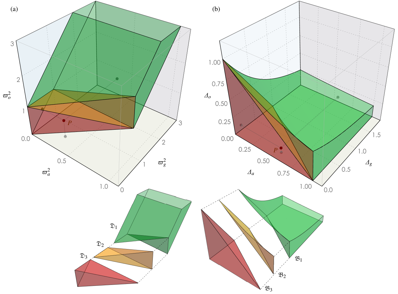
Figure 5: Three-dimensional domains of spectral multi-compatibility: (a) domains \mathfrak{D}_3 (red), \mathfrak{D}_2 (yellow), \mathfrak{D}_1 (green) in the space of (square) spectral bounds \varpi^2 = \{\varpi_a^2, \varpi_g^2, \varpi_o^2\} ; (b) domains \mathfrak{B}_3 (red), \mathfrak{B}_2 (yellow), \mathfrak{B}_1 (green) in the space of spectral bandwidths \mathcal{A} = \{\mathcal{A}_a, \mathcal{A}_g, \mathcal{A}_o\} .
