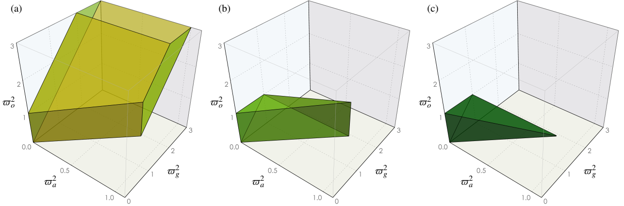
Figure 3: Three-dimensional domains of spectral compatibility in the space of (square) spectral bounds \boldsymbol{\omega}^2 = \{\omega_a^2, \omega_g^2, \omega_o^2\} : (a) domain \mathfrak{D}_A compatible with Criterion A , (b) domain \mathfrak{D}_B compatible with Criterion B , (c) domain \mathfrak{D}_C compatible with Criterion C .
