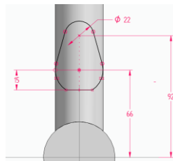
Fig. 6. Example of a robust and consistently alterable profile definition for the frontal boss consisting of a corrected set of basic dimensions and constraints.
