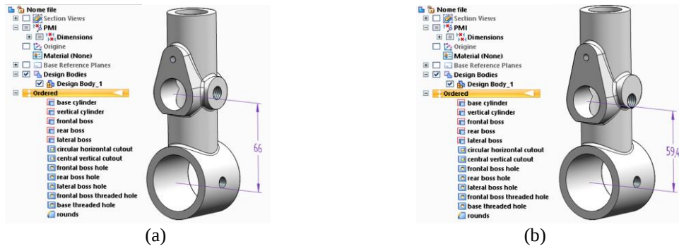
Fig. 21. Actual part where the type III dormant deficiency was discovered. From left to right: (a) CAD model, feature history, and dimensions of interest of latent type III dormant deficiency, (b) CAD model, feature history, and altered dimensions of interest of triggered type III dormant deficiency.
