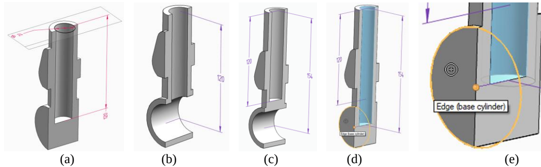
Fig. 11. Example of an extrusion option definition that contains inter-feature dependency errors. From left to right: (a) initial dimension and definition of extrusion option used for the central vertical cutout, (b) cross-section of the correctly created CAD model up to the modeling stage where the vertical and horizontal cutouts were created, (c) cross-section of the re-created CAD model shape exhibiting symptoms of a type II dormant deficiency, (d) cross-section of the correctly re-created CAD model using an alternative extrusion option that is based on a snap point, (e) enlarged cross-section of the topological/geometric condition related to the alternative extrusion option that is based on a snap point.
