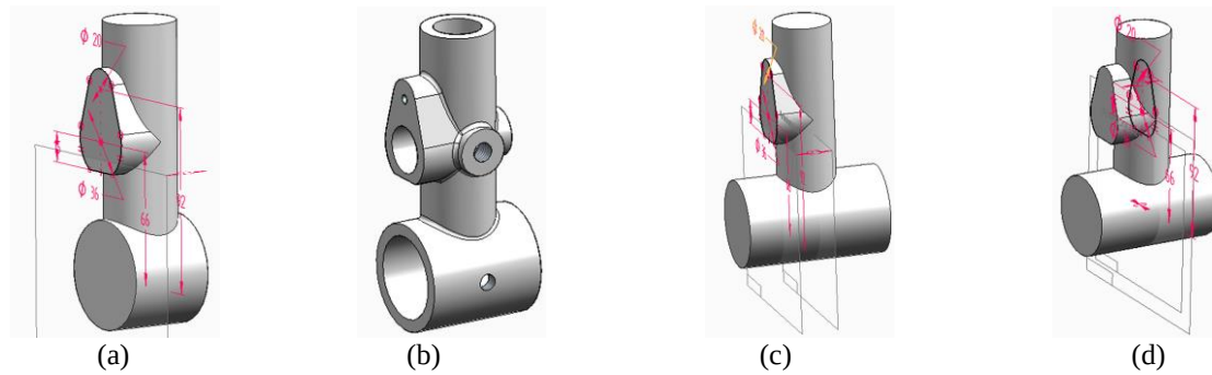
Fig. 7. Example of reference plane selection containing related inter-feature dependency errors. From left to right: (a) initial reference plane selection used for the frontal boss plane, (b) re-created CAD model shape exhibiting symptoms of a type III dormant deficiency after the base cylinder length has been changed, (c) correct reference plane selection for the frontal boss plane, (d) alternative correct reference plane selection for the frontal boss plane.
