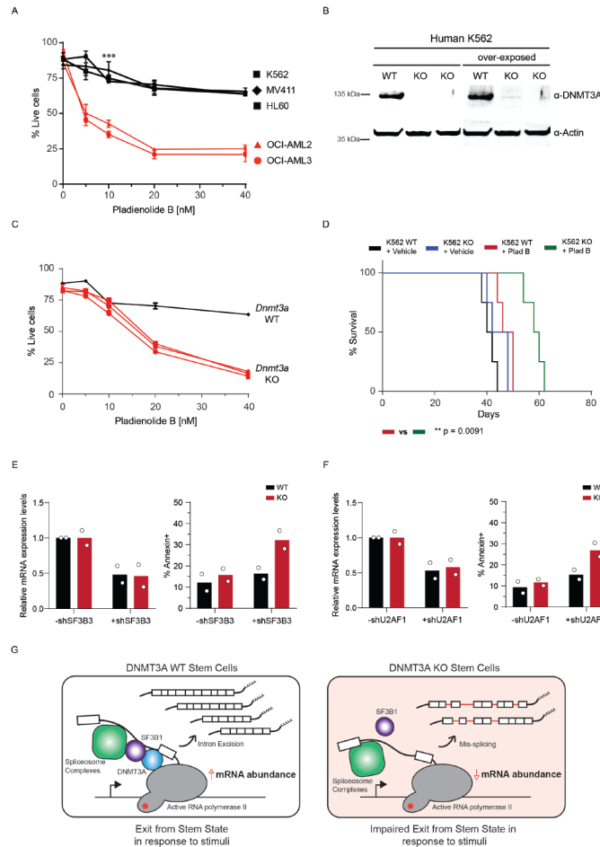
Extended Data Fig. 10. DNMT3A mutant leukemias are sensitive to splicing inhibition with Pladienolide B
