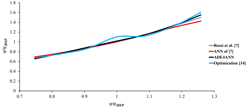
Figure 12: Non-dimensional characteristic curves comparison
