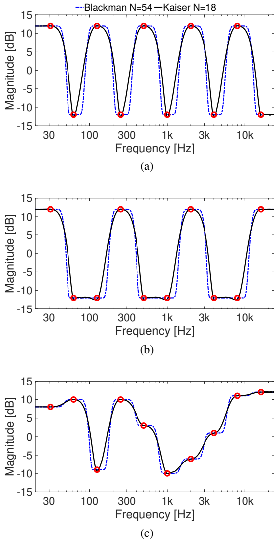
Fig. 11. Magnitude response of the proposed equalizer for two different prototype filters, considering (a) the zigzag configuration ( \pm 12 dB), (b) the gains [12 -12 -12 12 -12 -12 12 -12 -12] dB, and (c) the arbitrary gains [8 10 -9 10 3 -10 -6 1 11 12] dB.
