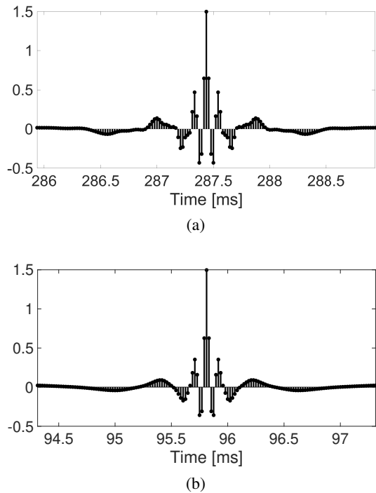
Fig. 12. Impulse response of the proposed equalizer designed using (a) the Blackman window with an order of N = 54 and (b) the Kaiser window with an order of N = 18 for the configuration of Fig. 11(a).
