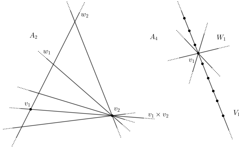
FIGURE 4. Non-smooth reducible (1,1) -surfaces are singular along an element of \bar{\mathcal{V}} : either a curve L_{q,m} for the case A_2 or the union of two intersecting fibers \pi_1^{-1}(q) \cup \pi_2^{-1}(m) for A_4 .
