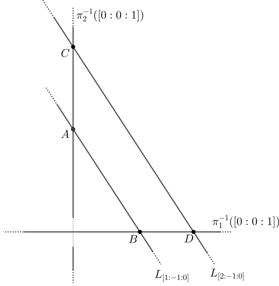
FIGURE 6. Intersection of S and j(S) . Notice how S \cap j(S) is a connected set of two (1, 1) -curves and two canonical (skew) fibers.
