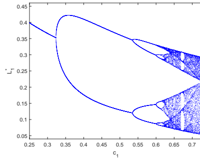
Figure 4: Bifurcation diagram on varying c_1 \in (0.25, 0.73) . Parameters values: \gamma = 0.12 , \alpha = 2.02 , r = 1.59 , c_2 = 0.35 , and i.c. L_{1,0} = 0.15 , L_{2,0} = 0.63 .
