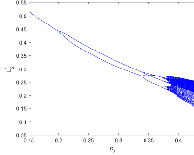
Figure 3: Bifurcation diagram on varying c_2 \in (0.15, 0.43) . Parameters values: \gamma = 0.12 , \alpha = 2.35 , r = 1.5 , c_1 = 0.34 , and i.c. L_{1,0} = 0.3 , L_{2,0} = 0.5 .
