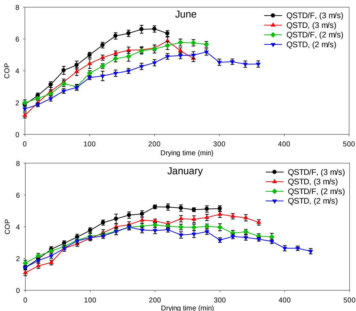
Fig. 10. Time dependent variation of COP values
