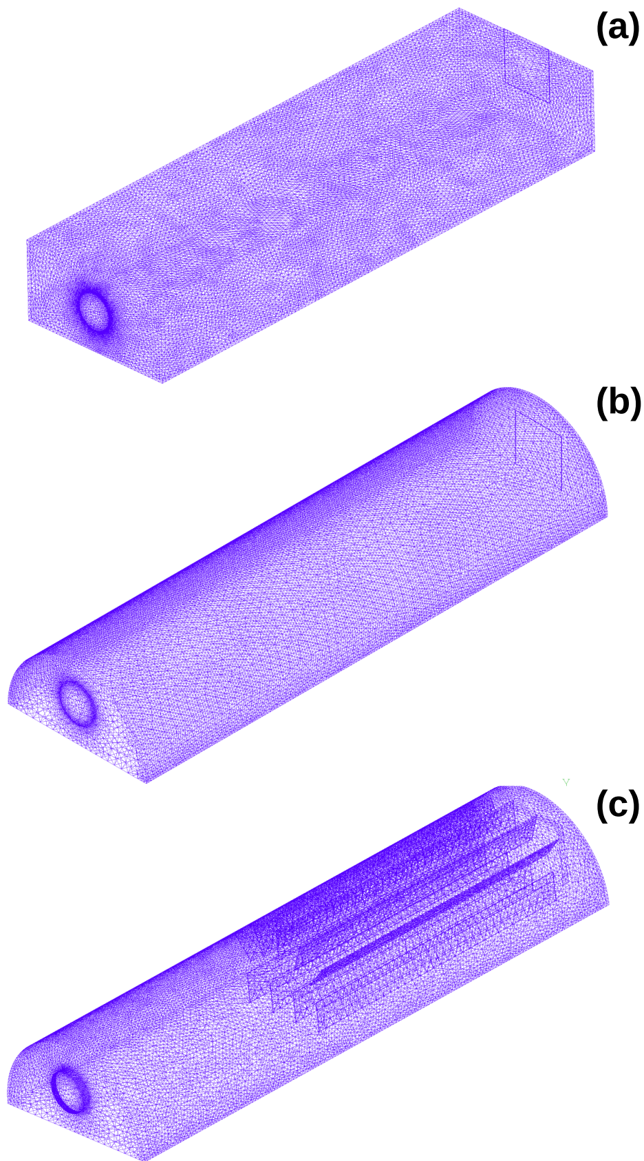
Fig. 3. The generated mesh for three tunnel dryers
