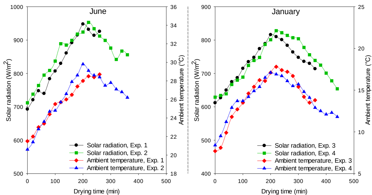
Fig. 9. Time dependent variation of solar radiation and ambient temperature values
