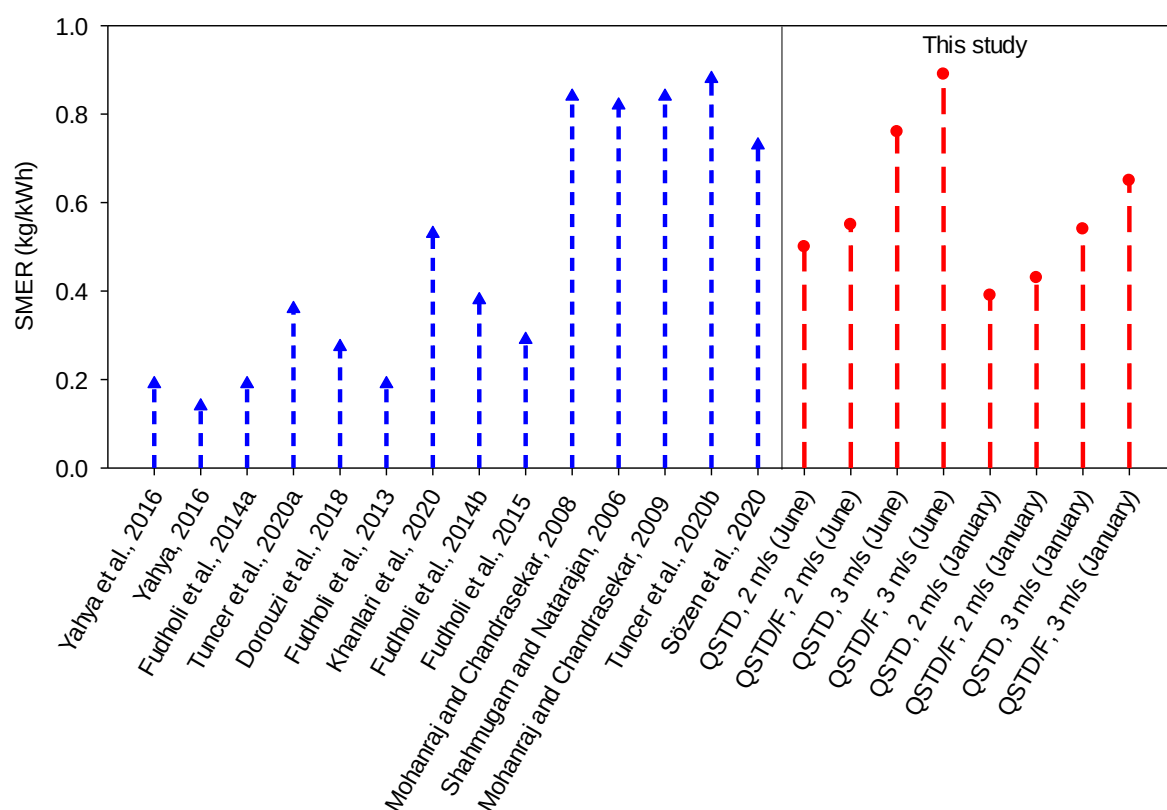
Fig. 13. Comparison of obtained SMER values with available studies about solar dryers in the literature
