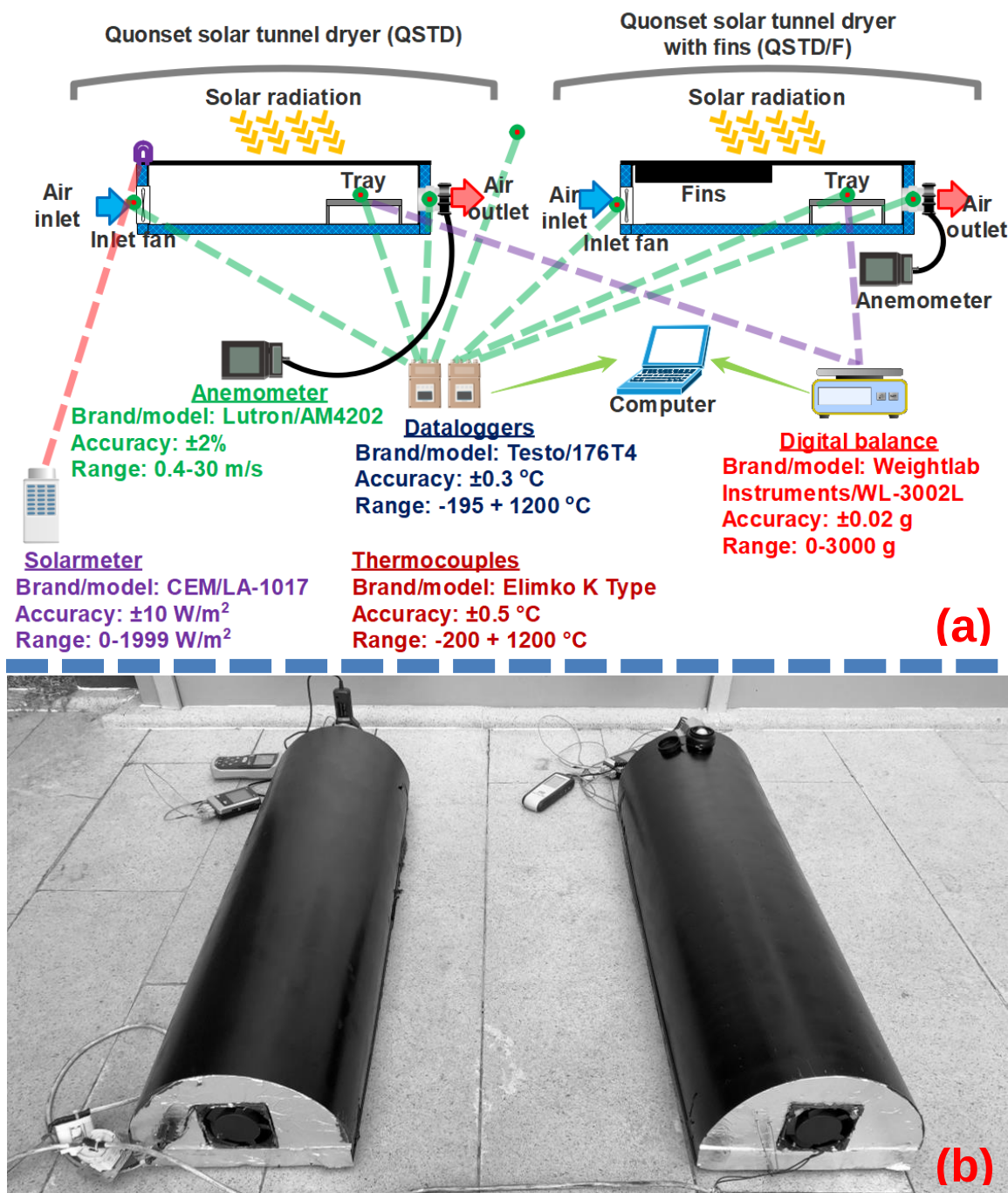
Fig. 5. Experimental setup of tunnel dryers; a) Schematic diagram, (b) Photograph
