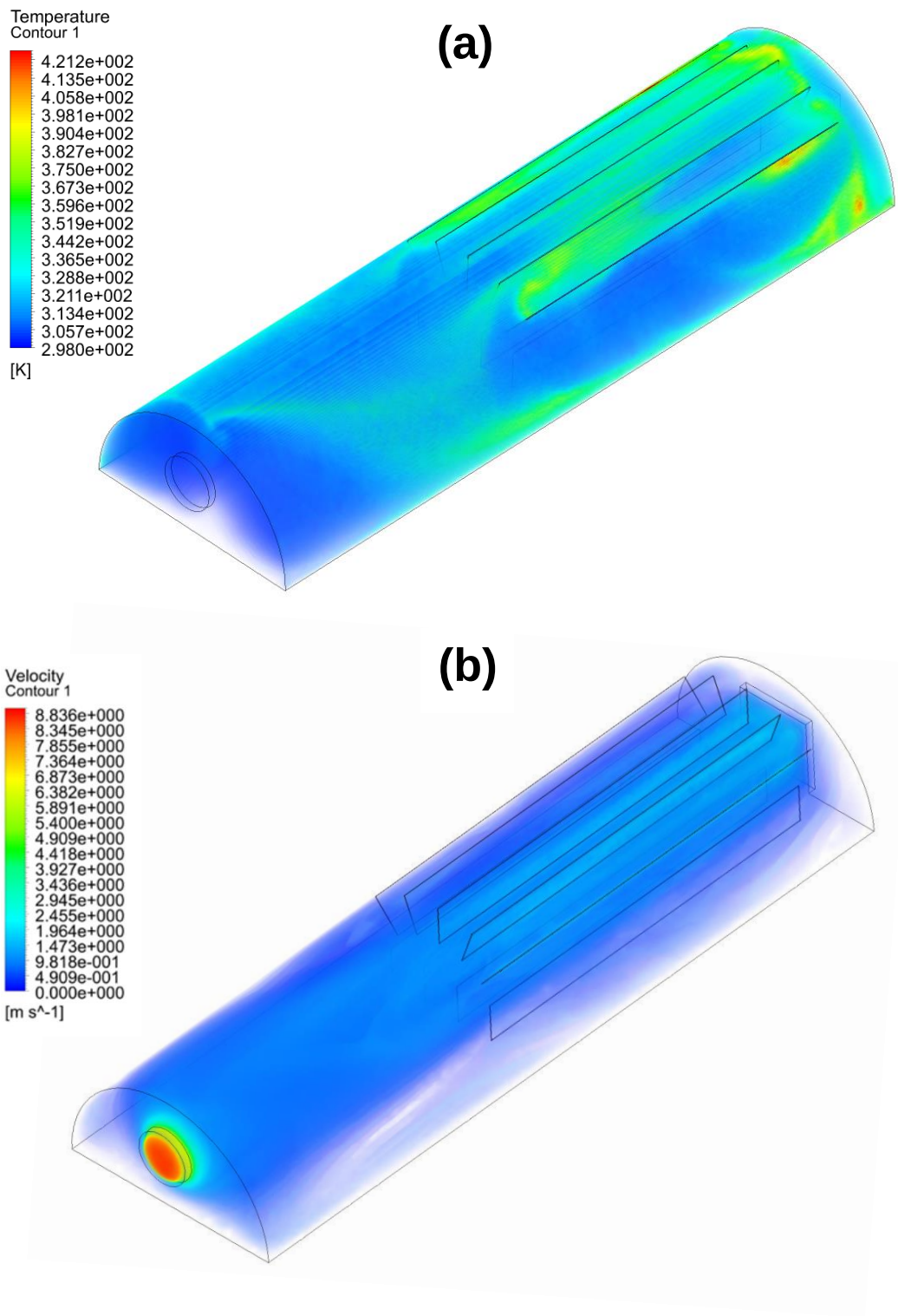
Fig. 8. Volume rendering images of QSTD/F at 2 m/s air velocity; a) temperature, b) velocity
