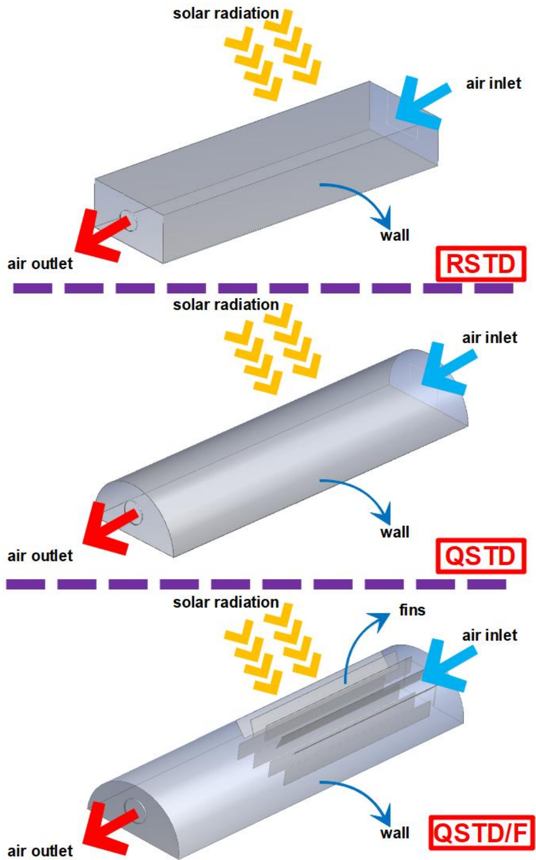
Fig. 2. Geometry and boundary condition for solar tunnel dryers
