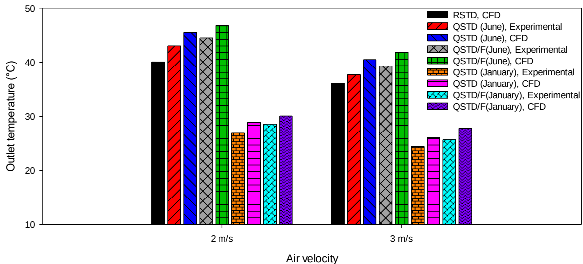
Fig. 15. Obtained numerical and experimental outlet temperature values
