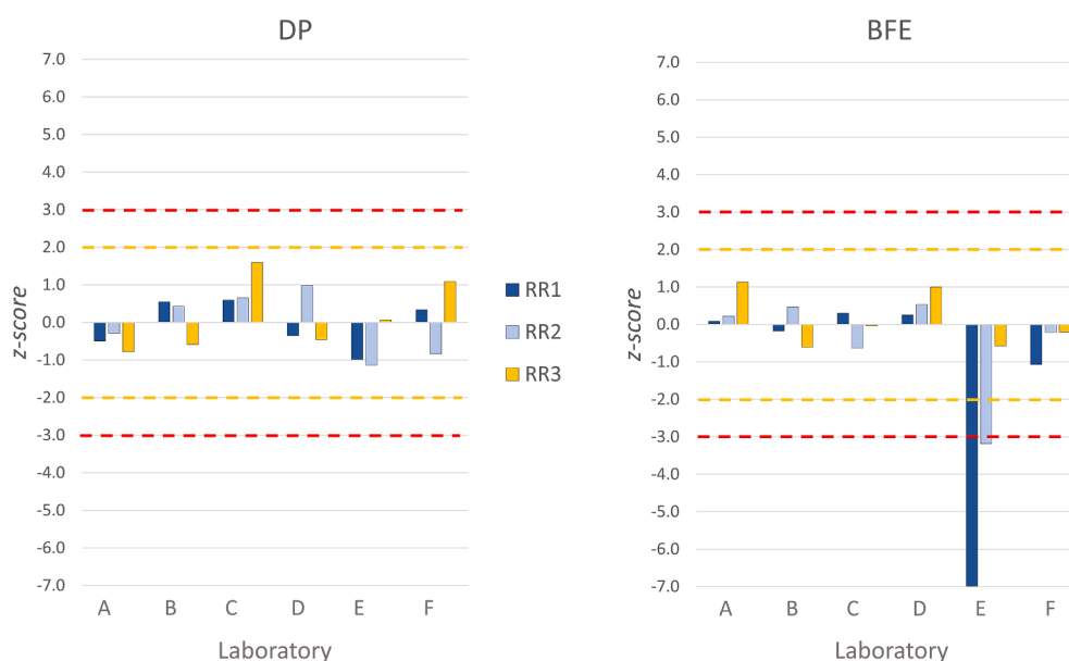
Fig. 8. Results of the proficiency test for all the participating labs for the DP (left) and BFE (right) measurements. Average z -score are indicated for each of the three mask types. Yellow and red dashed line represents thresholds for alert and intervention actions. (For interpretation of the references to colour in this figure legend, the reader is referred to the web version of this article.)
