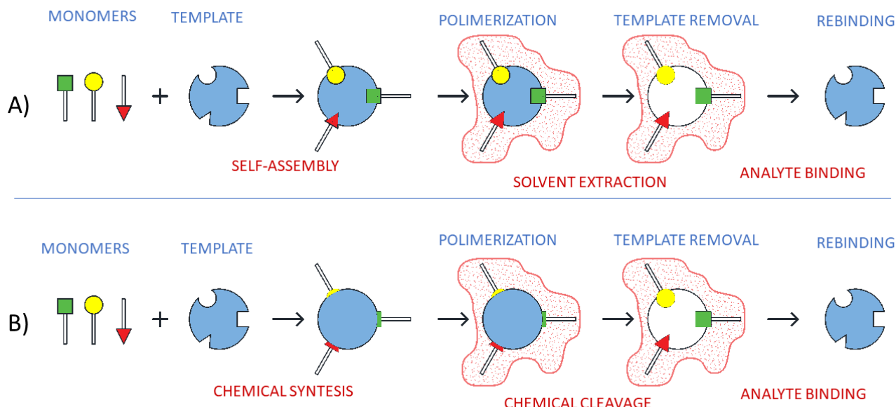
Fig. 2. Polymerization steps of MIPs through a) non-covalent b) covalent (adapted from [89]).
