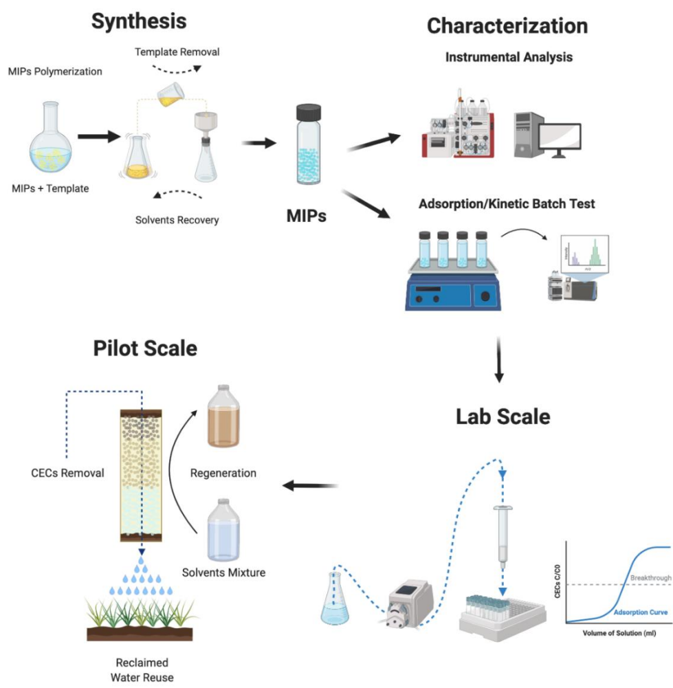
600 601 Fig. 3. A possible upscaling pathway for MIPs application to wastewater treatment for enhanced 602 CECs removal and safe water reuse in irrigation/fertigation.
