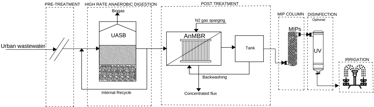
Fig. 4. A possible configuration for integrating MIP columns to urban water cycle facilities for enhanced CECs removal and enabling safe water reuse in irrigation/fertigation. This configuration is currently being developed under the PRIMA/H2020 Project “FIT4REUSE” (fit4reuse.org).
