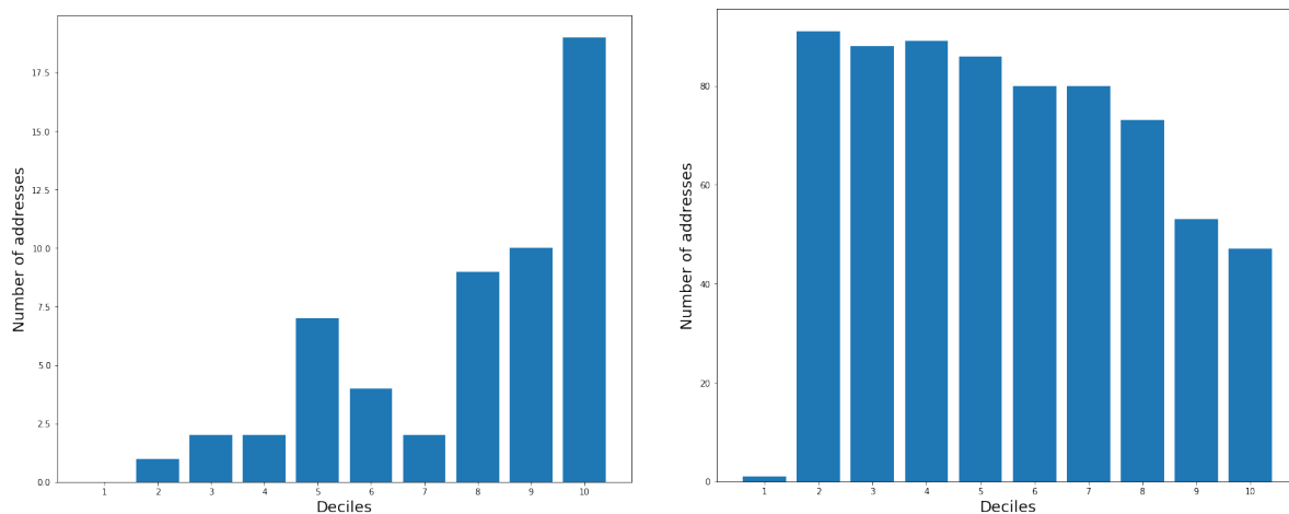
Figure 10: Distribution of the addresses of \mathcal{S}^T (at left) and \mathcal{M}^T (at right) against the number of transactions of T_{Pre}^T
