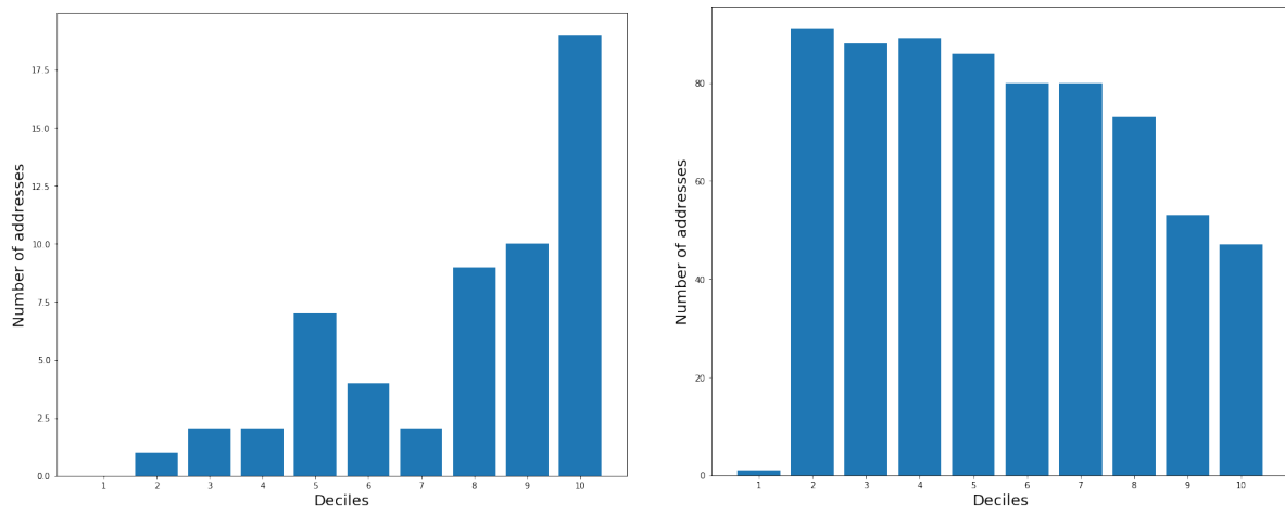
Figure 10: Distribution of the addresses of S^T (at left) and \mathcal{M}^T (at right) against the number of transactions of T_{Pre}^T
