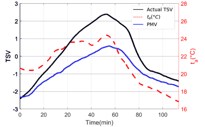
Fig. 13. Average trend of TSV and PMV against air temperature during Experiment 3, for all the users.
