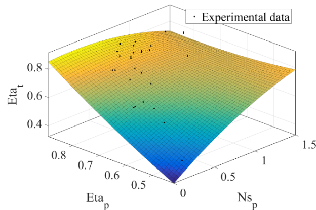
Fig. 3. 3D plot of \eta_t as a function of N_{Sp} and \eta_p
